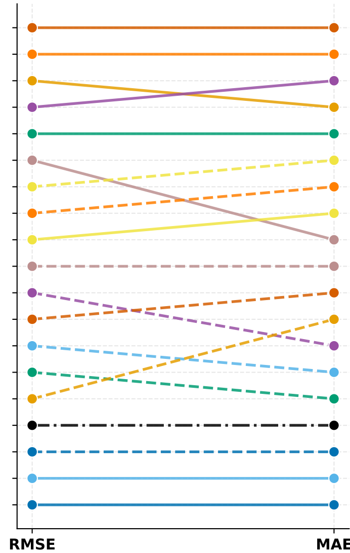
DiaTrend
