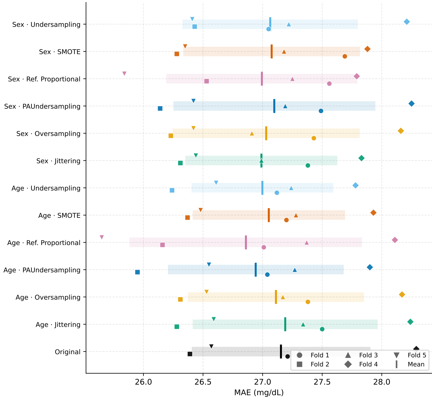
Fold consistency — ReplaceBG | MAE · All Ranges
