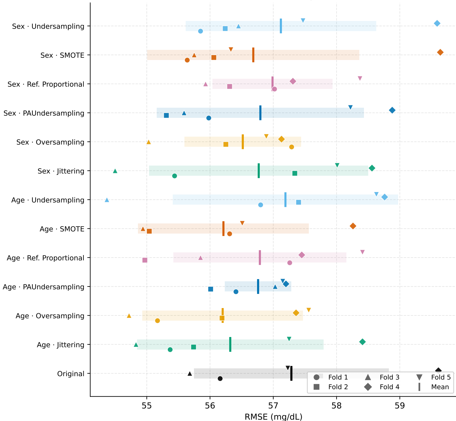
Fold consistency — ReplaceBG | RMSE · Hypo L2
