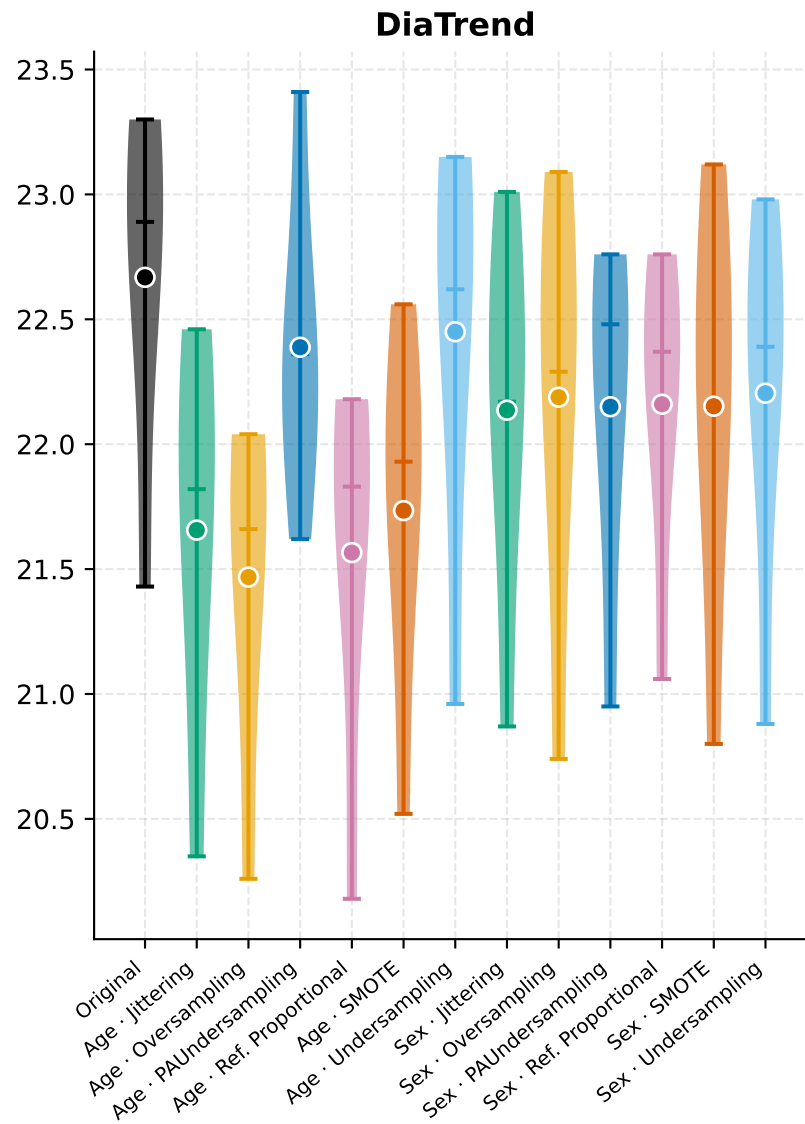
Distribution across folds — MAE · In Range | ● = mean, — = median
