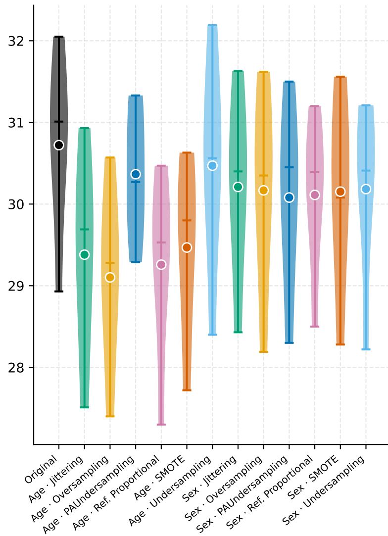
DiaTrend
