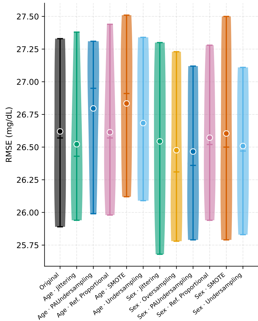
T1DGranada
