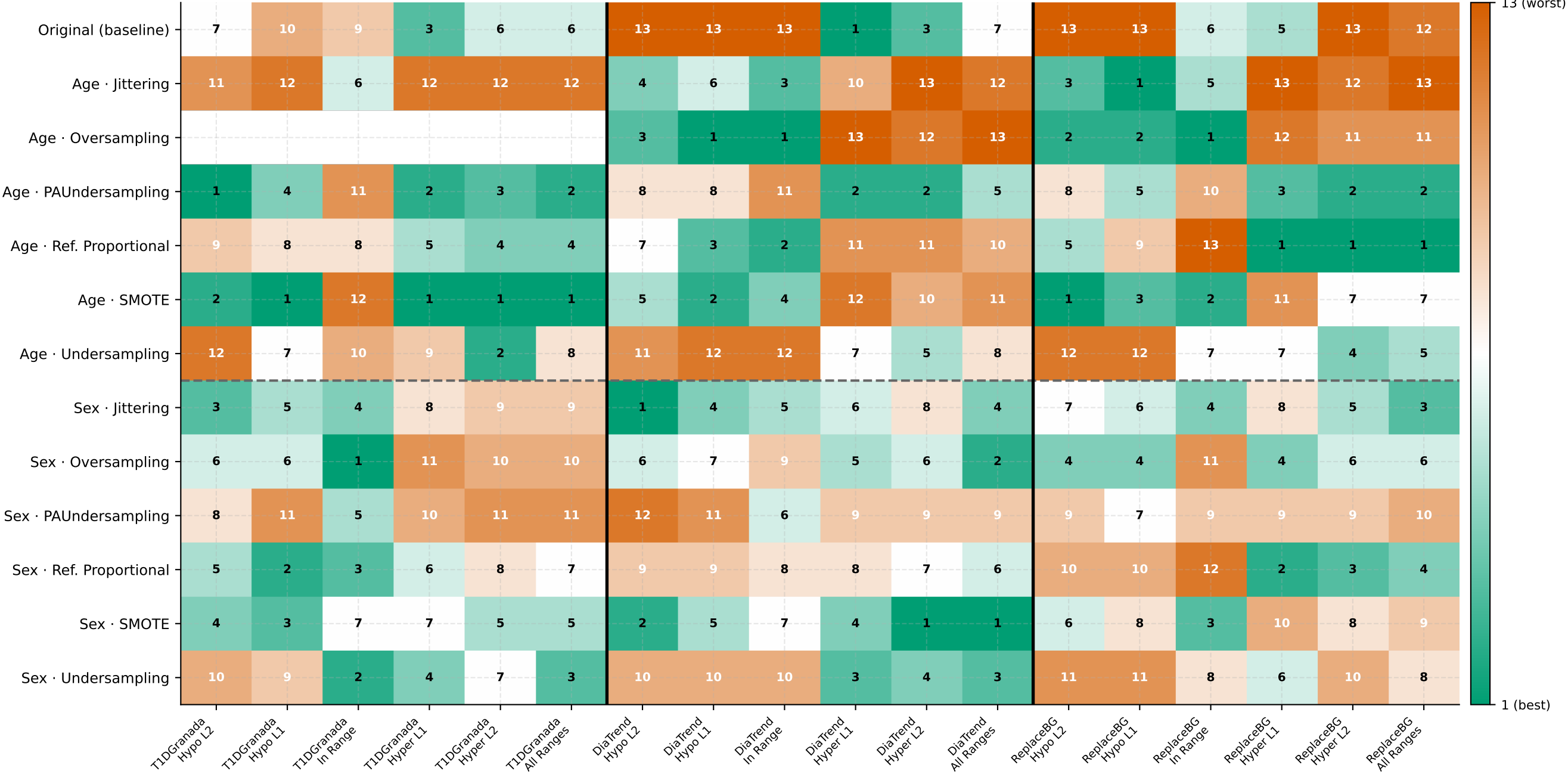
Ranking position by technique × dataset × glucose range | MAE
