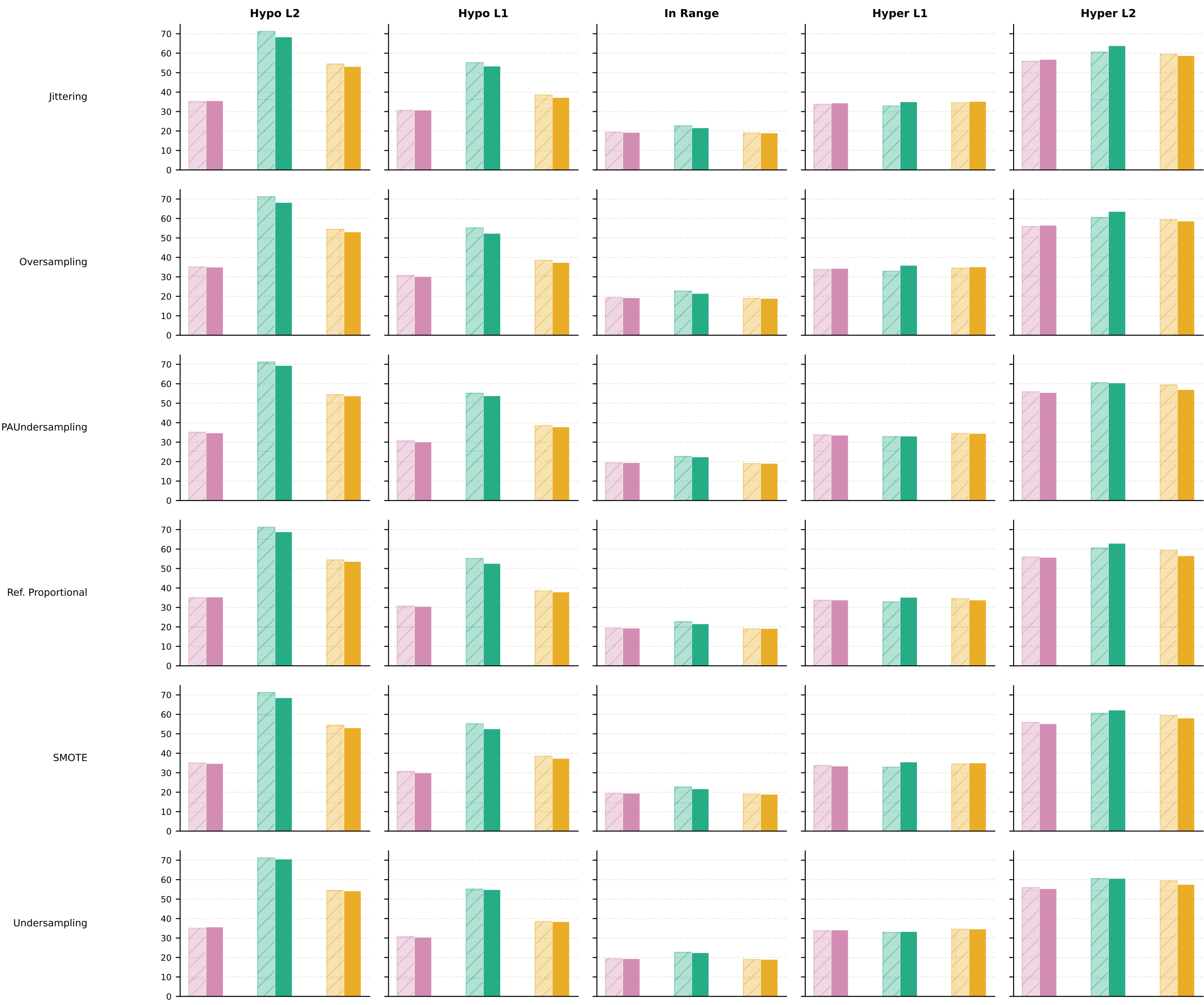
Small multiples — MAE by technique × glucose range Row = technique | Column = glucose range | Hatched = baseline
