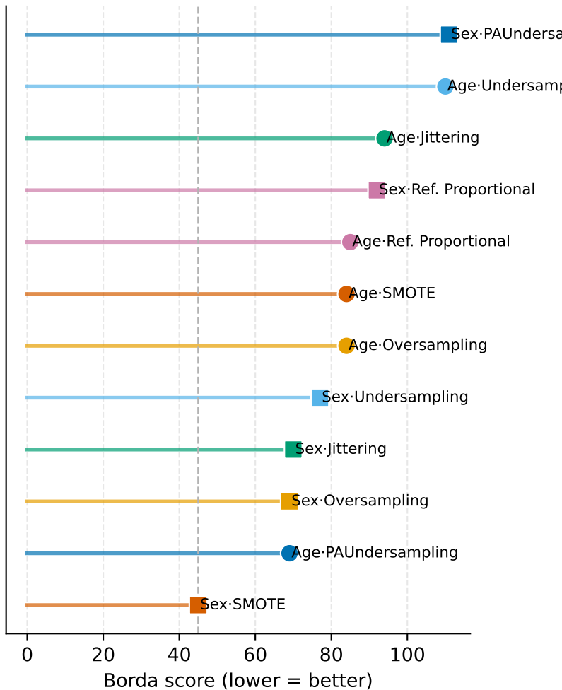
DiaTrend
