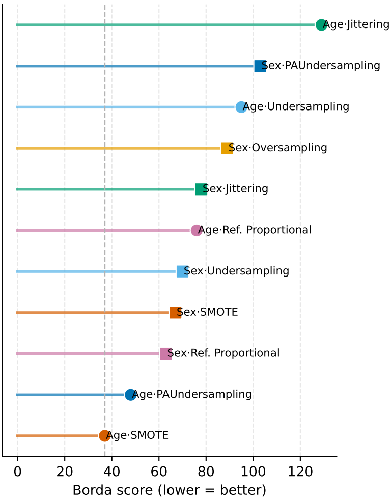
T1DGranada
