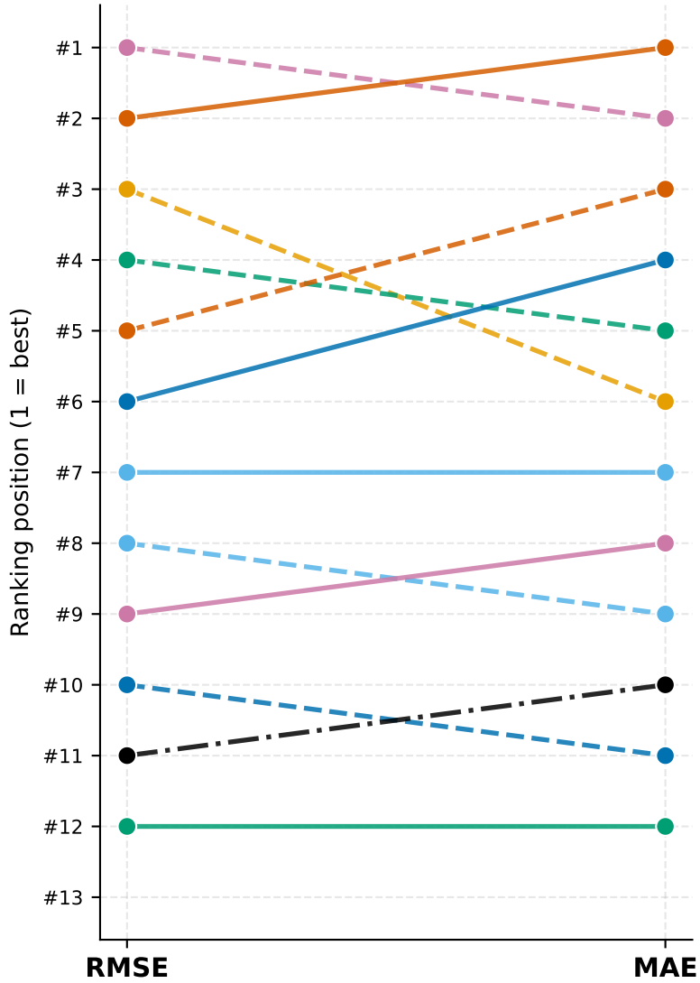
T1DGranada
