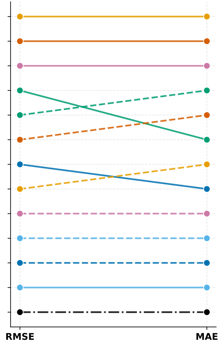
DiaTrend
