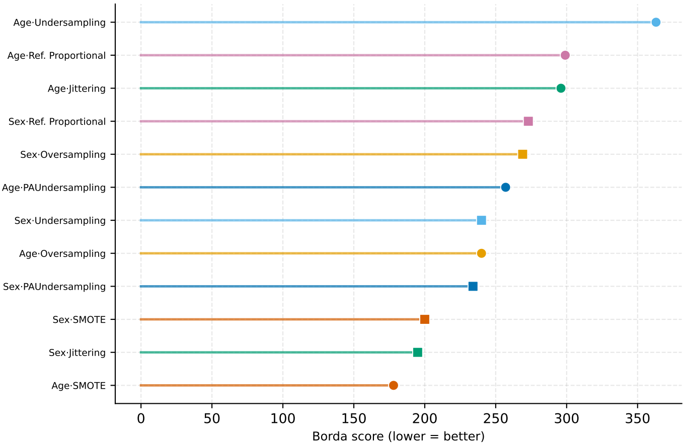
B | Aggregate Borda ranking (lower = better)
