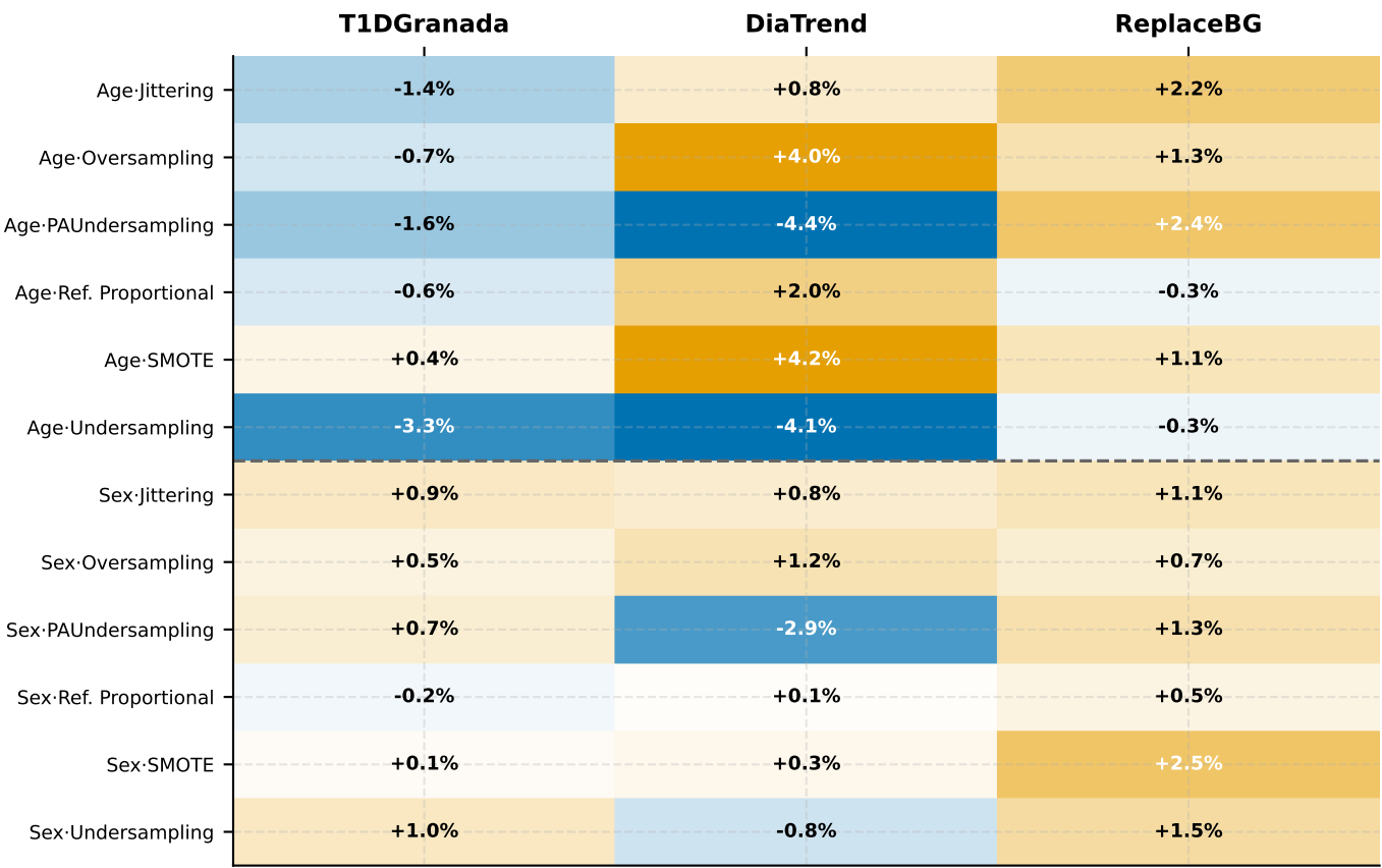
D | RMSE improvement vs. baseline (Hypo L1 · 54-69 mg/dL)
