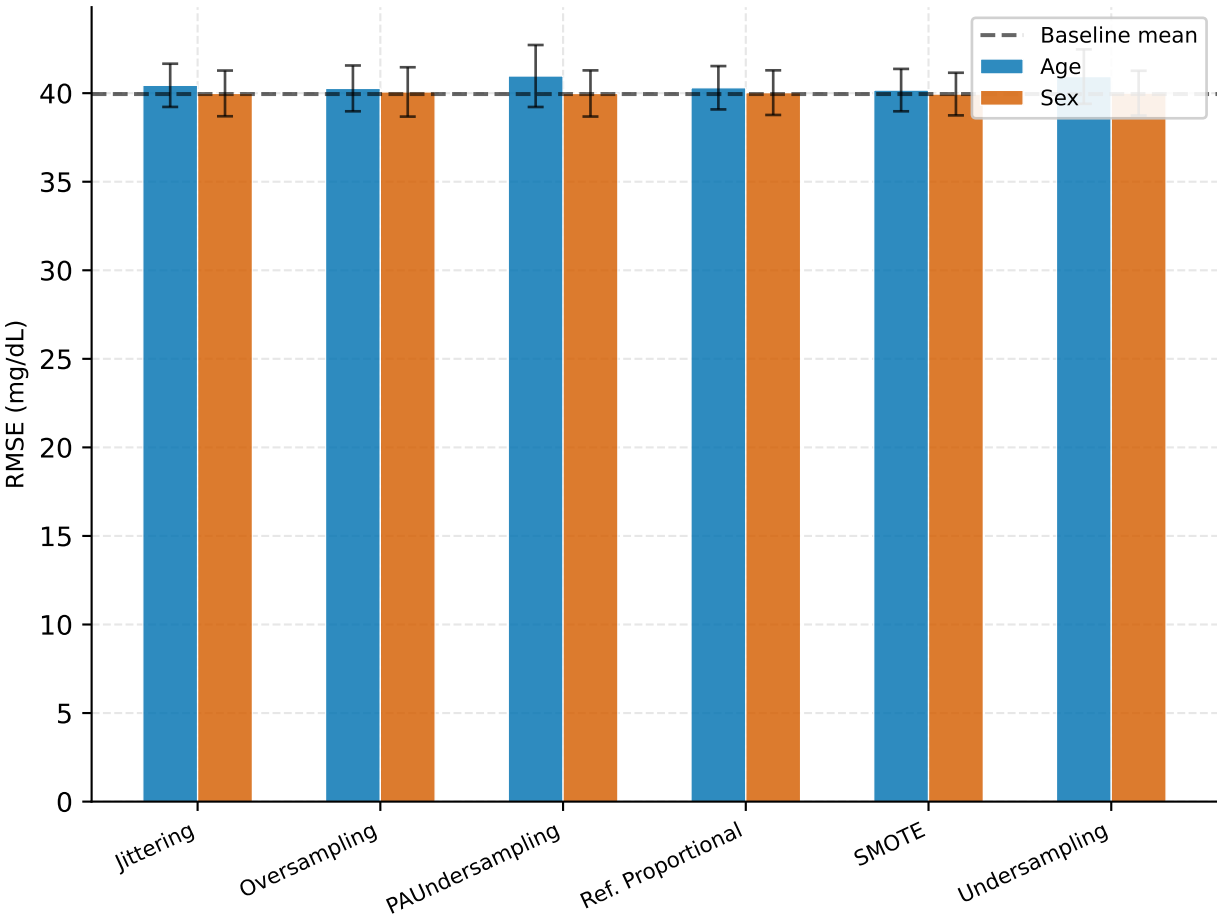
C | Mean RMSE by technique and dimension
