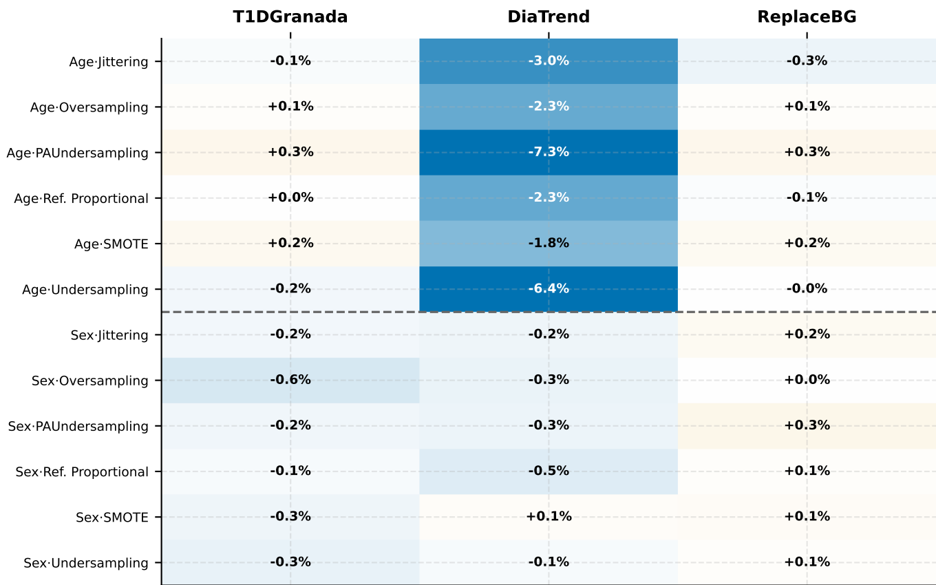
A | RMSE improvement vs. baseline (All ranges)
