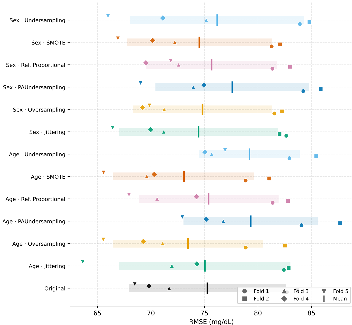
Fold consistency — DiaTrend | RMSE · Hypo L2
