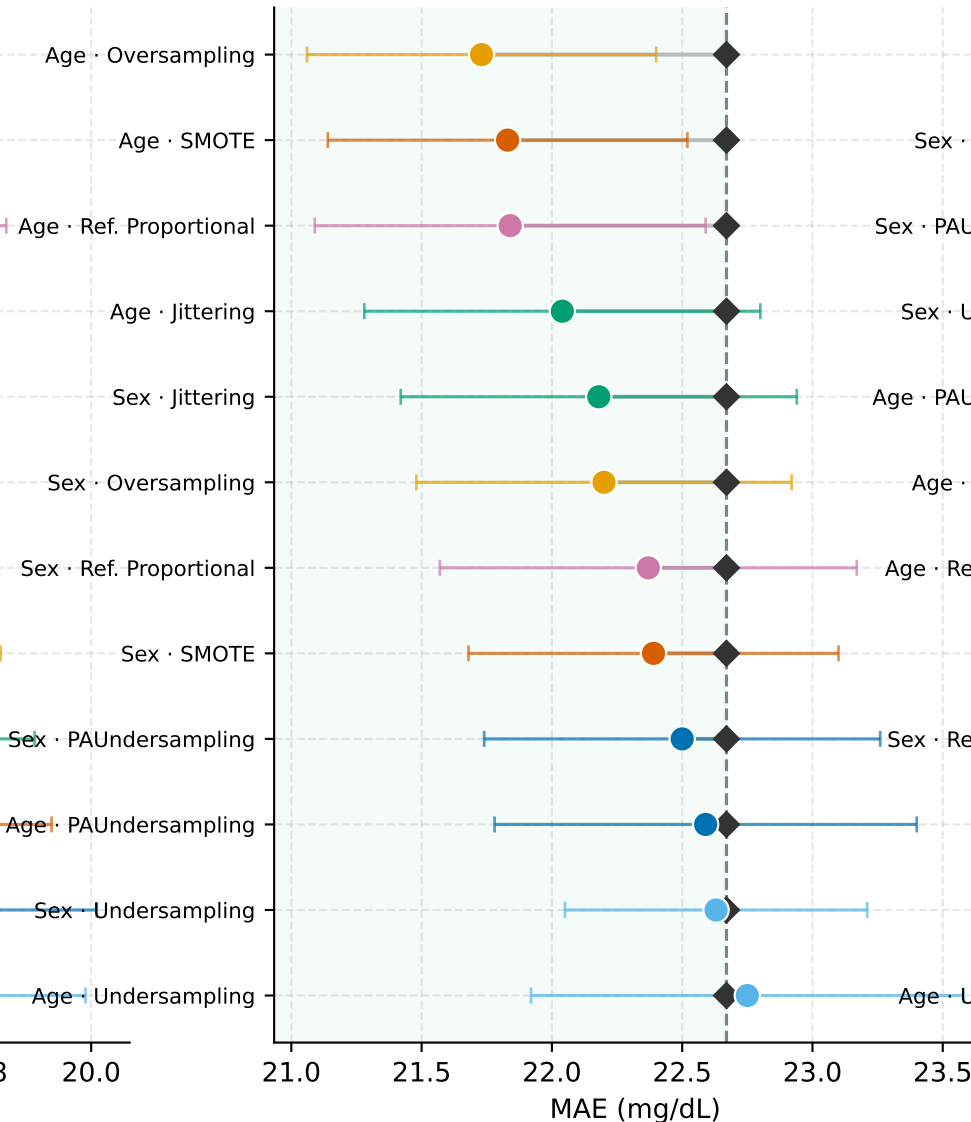
DiaTrend
