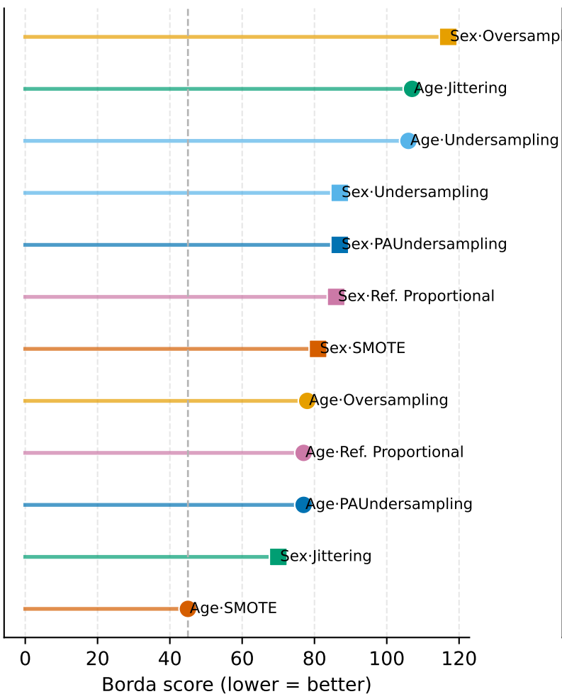
T1DGranada
