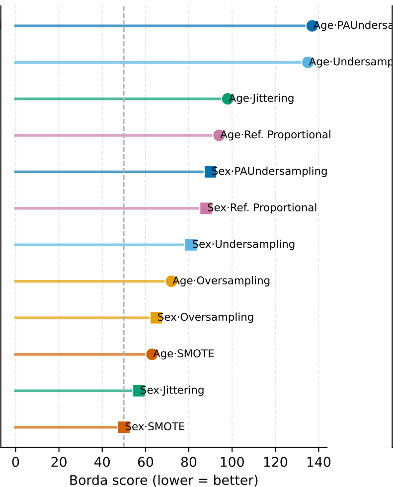
DiaTrend
