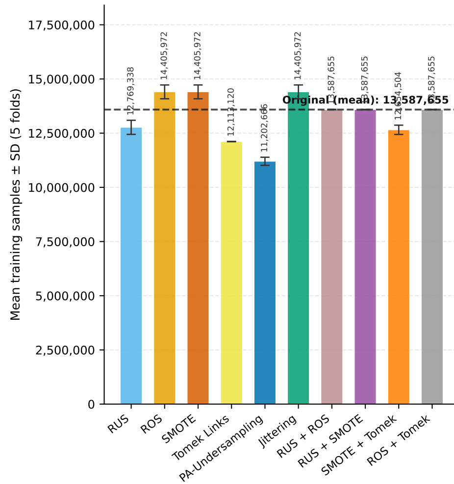
T1DGranada
