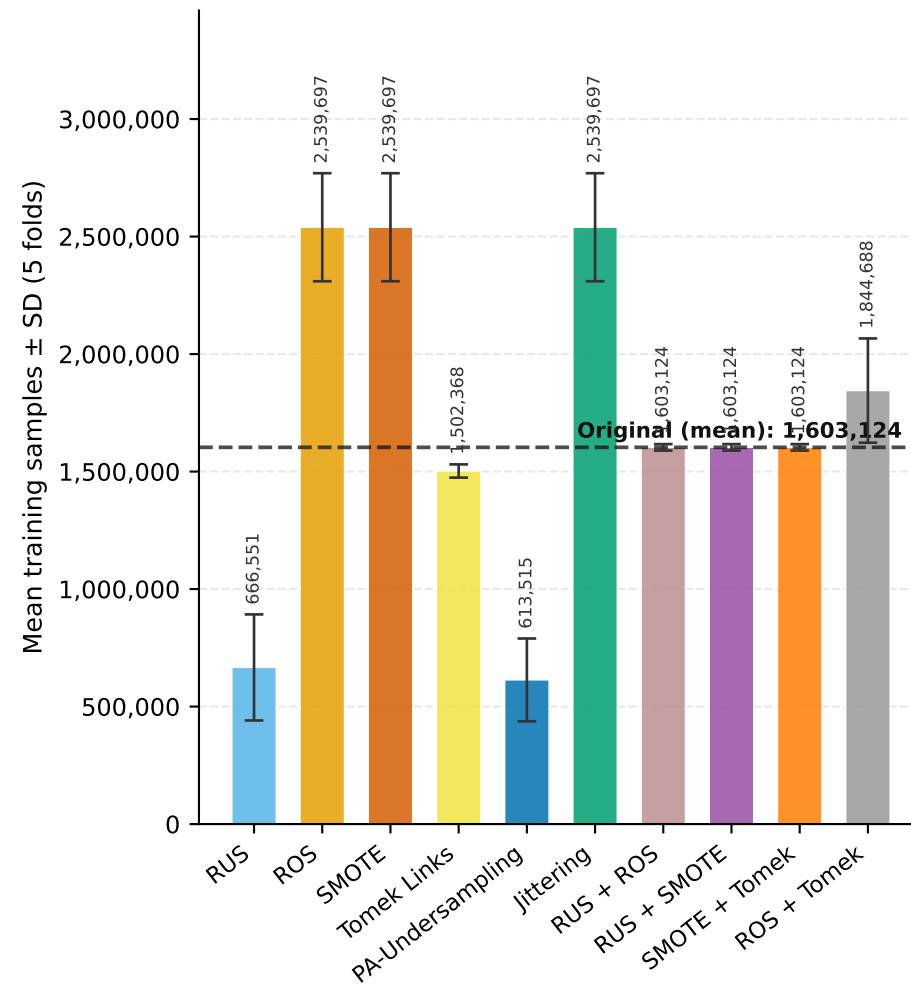
DiaTrend
