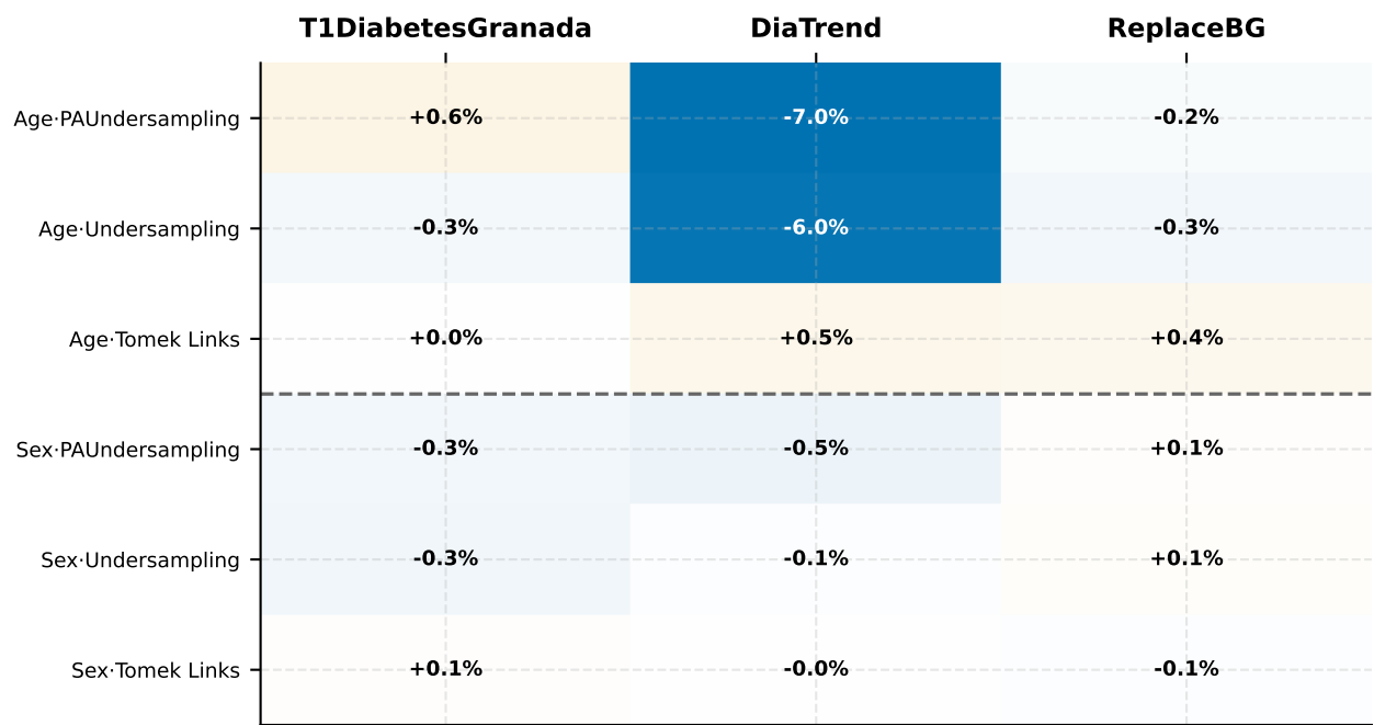
Undersampling: RMSE improvement
