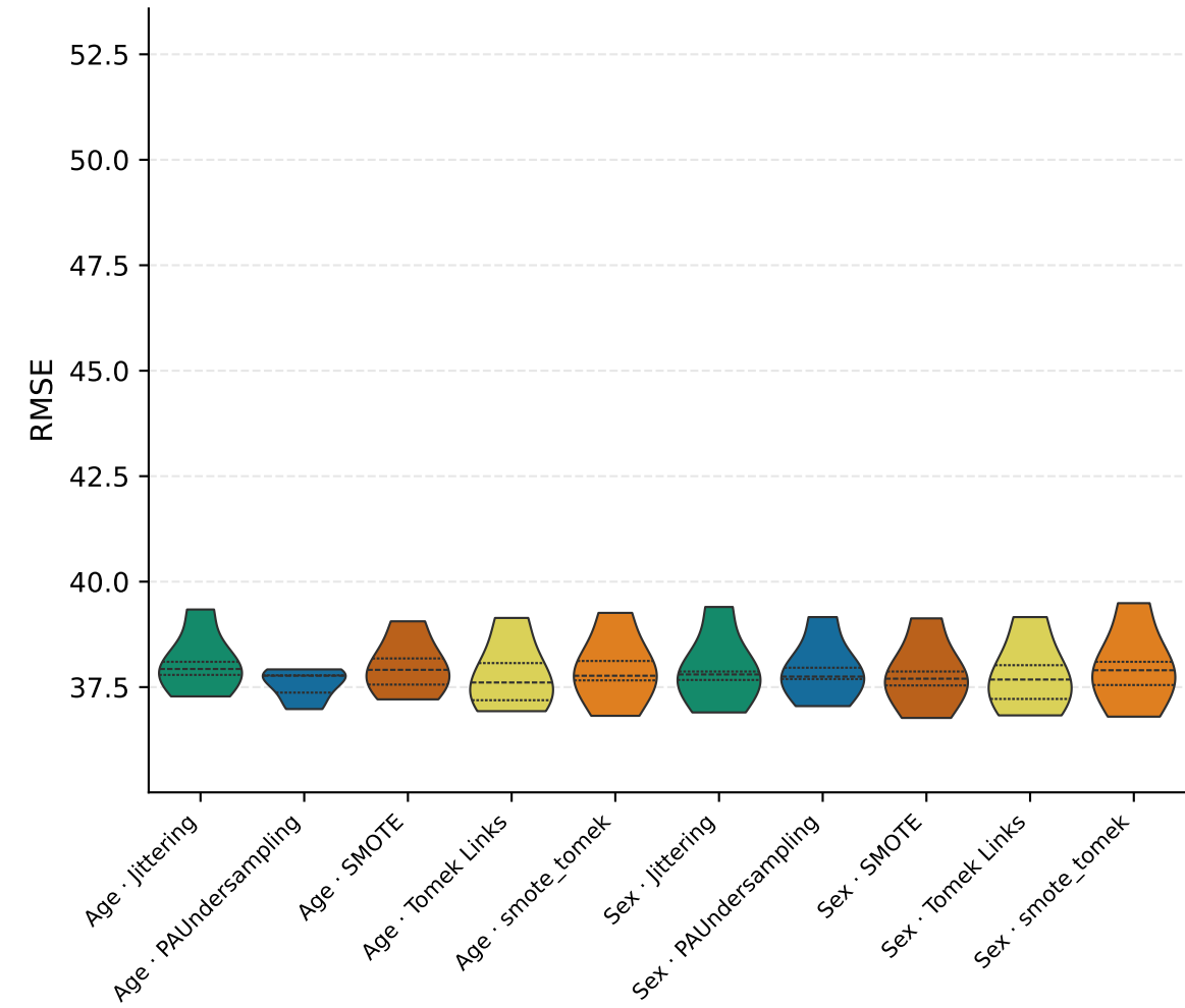
T1DiabetesGranada — RMSE · All Ranges
