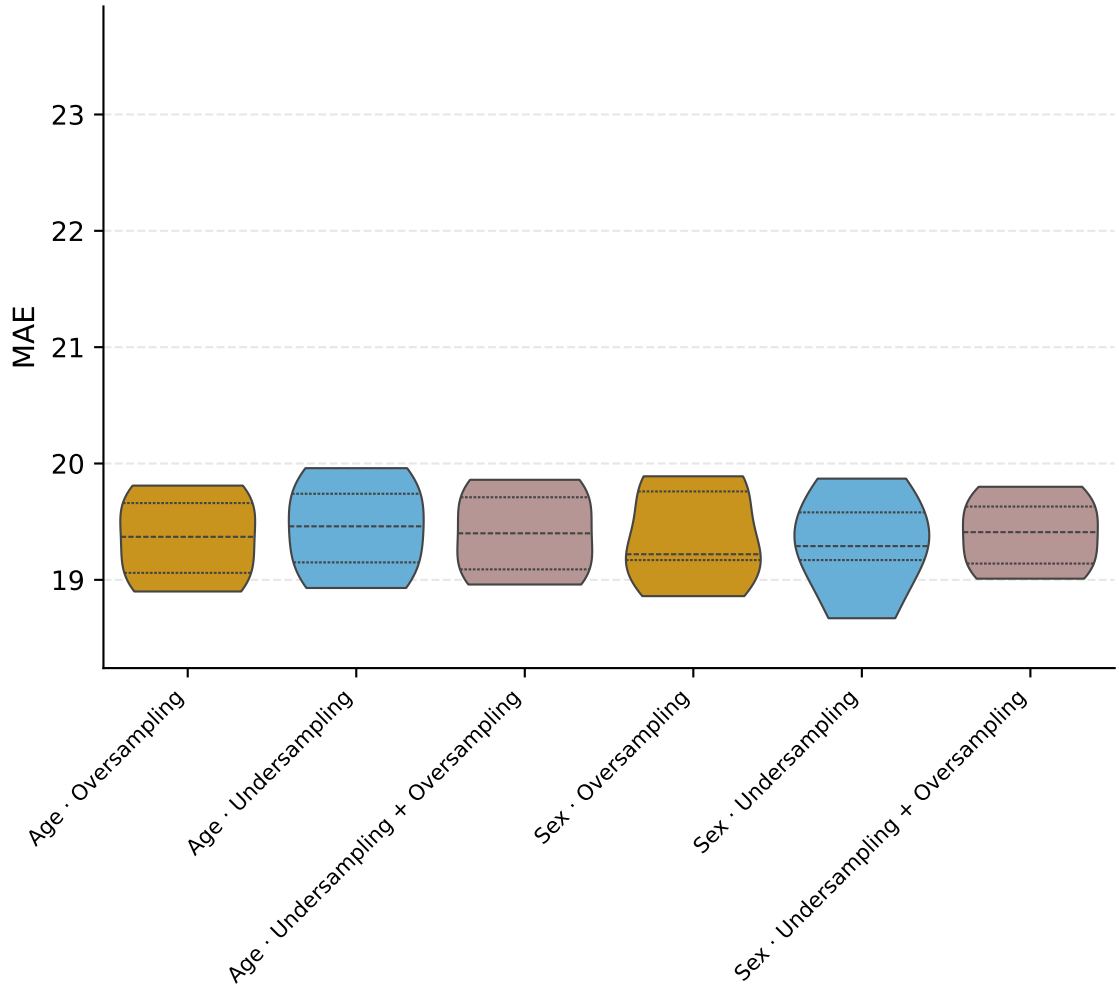
T1DiabetesGranada — MAE · In Range
