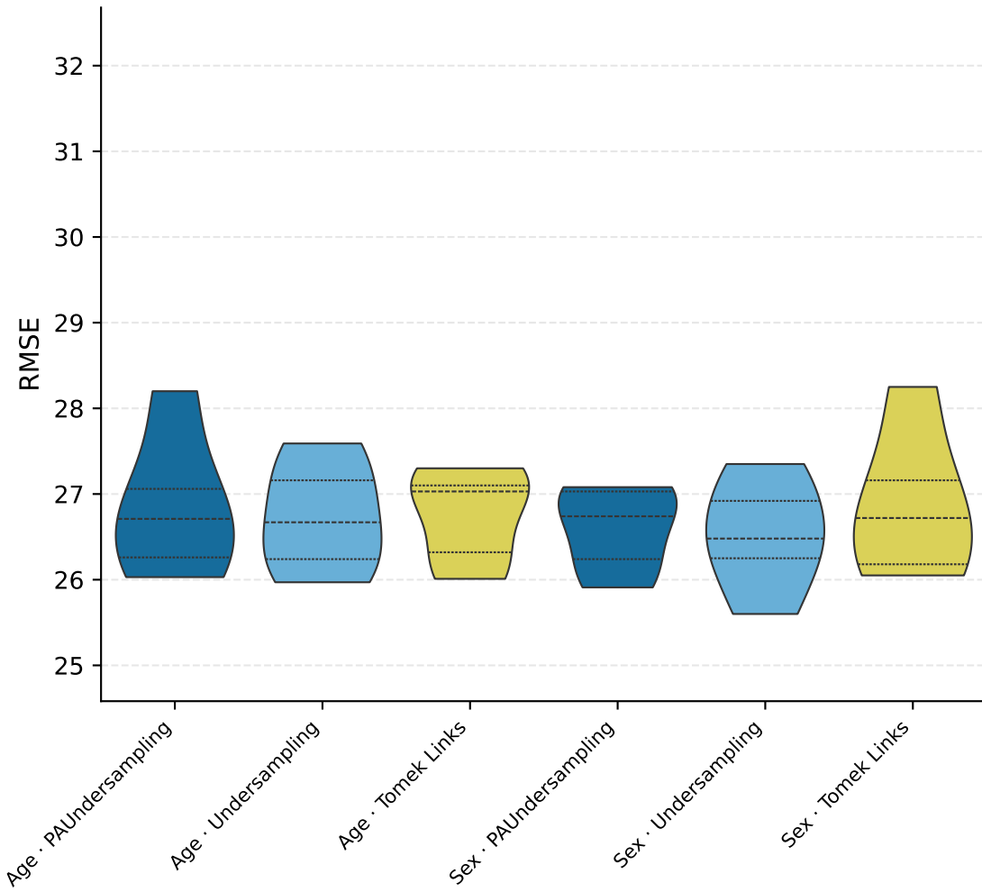
T1DiabetesGranada — RMSE · In Range
