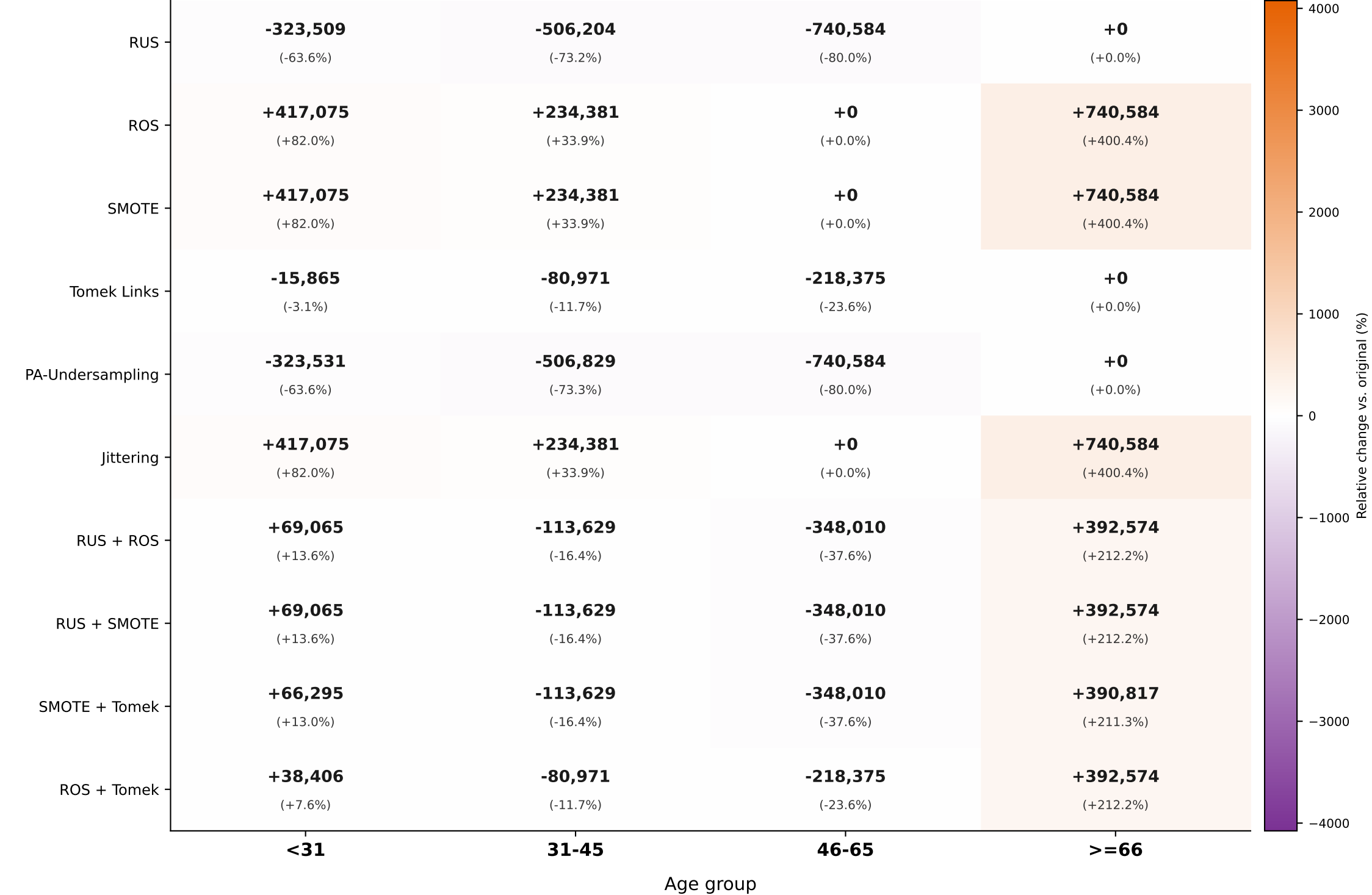
ReplaceBG · Balancing effect on train composition (Age dimension) Cell: mean Δsamples (bold) and Δ% across 5 folds | Purple = loss · Orange = gain
