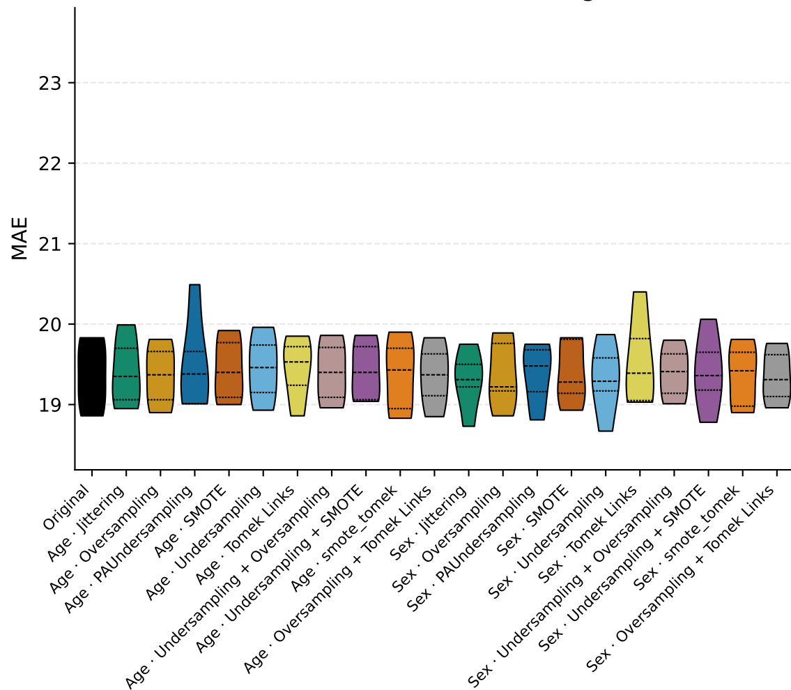
T1DGranada — MAE · In Range
