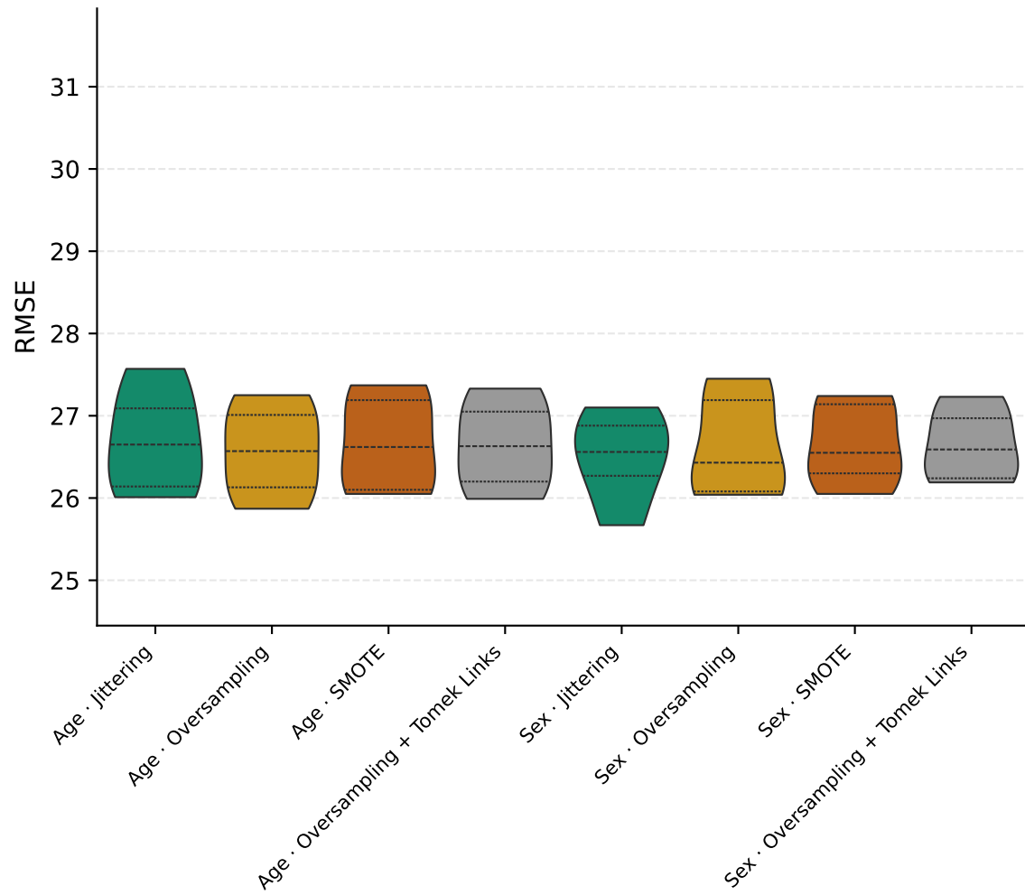
T1DGranada — RMSE · In Range
