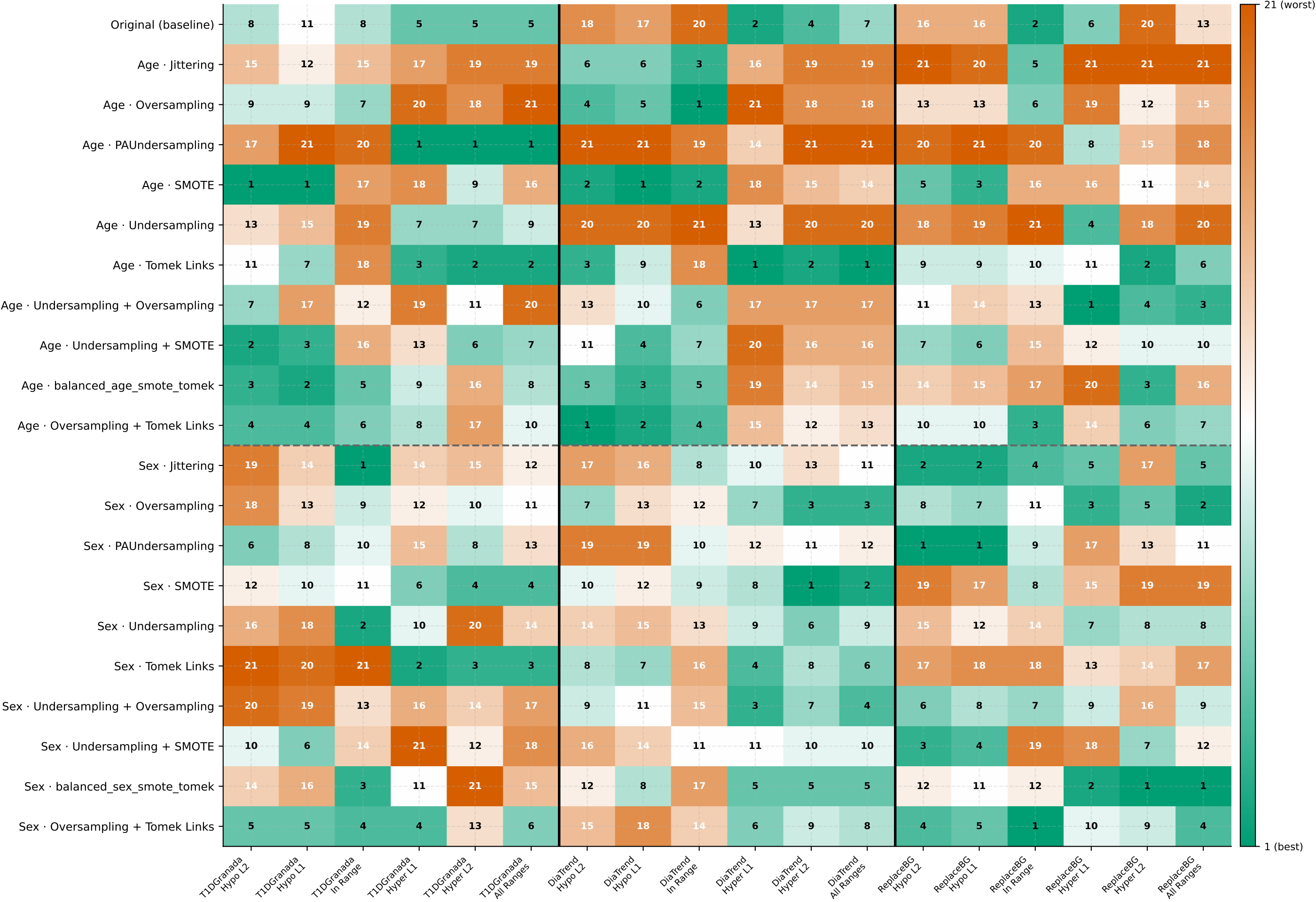
Ranking position by technique × dataset × glucose range | MAE
