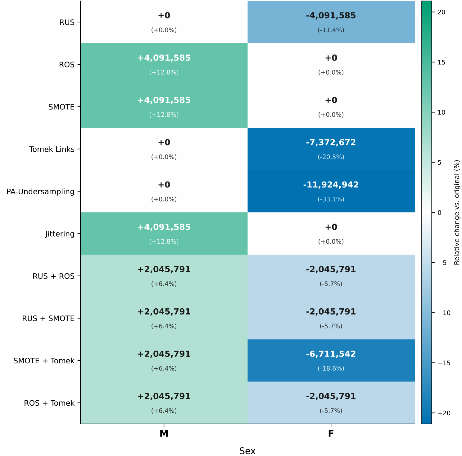
T1DGranada · Balancing effect on train composition (Sex dimension) Cell: mean \Delta samples (bold) and \Delta\% across 5 folds | Blue = loss · Green = gain
