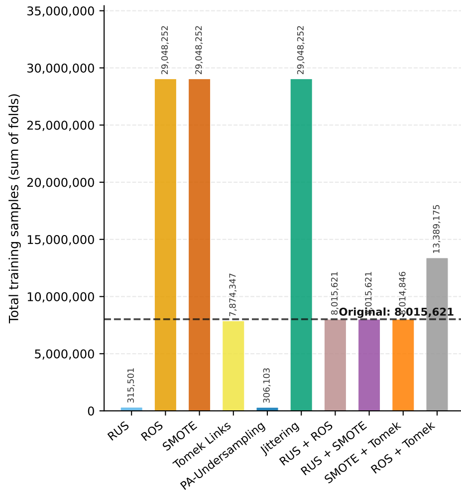
DiaTrend
