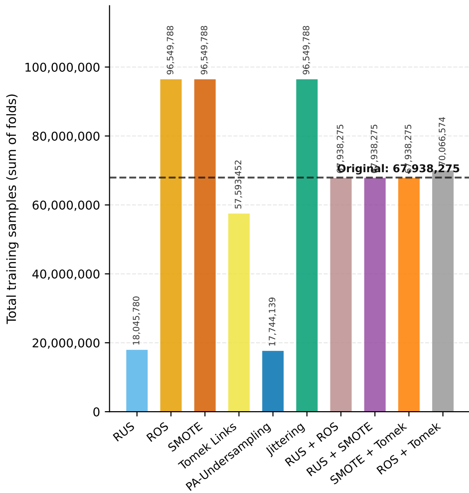
T1DGranada
