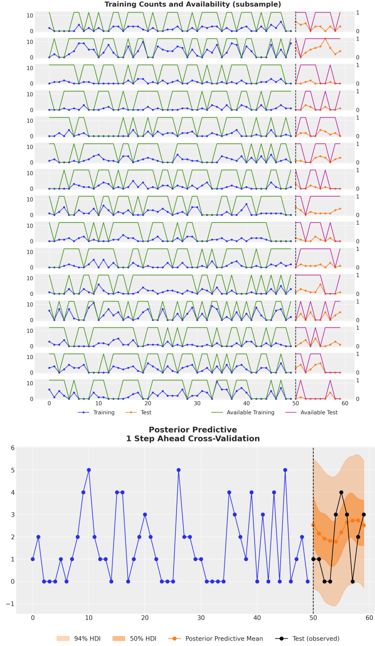
Figure 2: Top: an observed sales series with the corresponding availability mask. Long runs of zeros coincide with periods when the item was unavailable. Bottom: posterior predictive forecast from the availability-aware TSB model. The model recovers latent demand from intermittent and partially censored observations.
