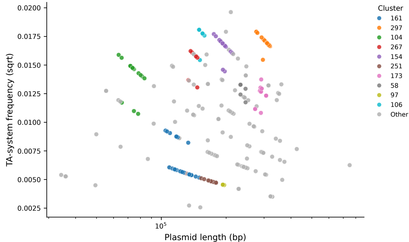
Colored by MobMess cluster (top 10, n = 300 plasmids)
