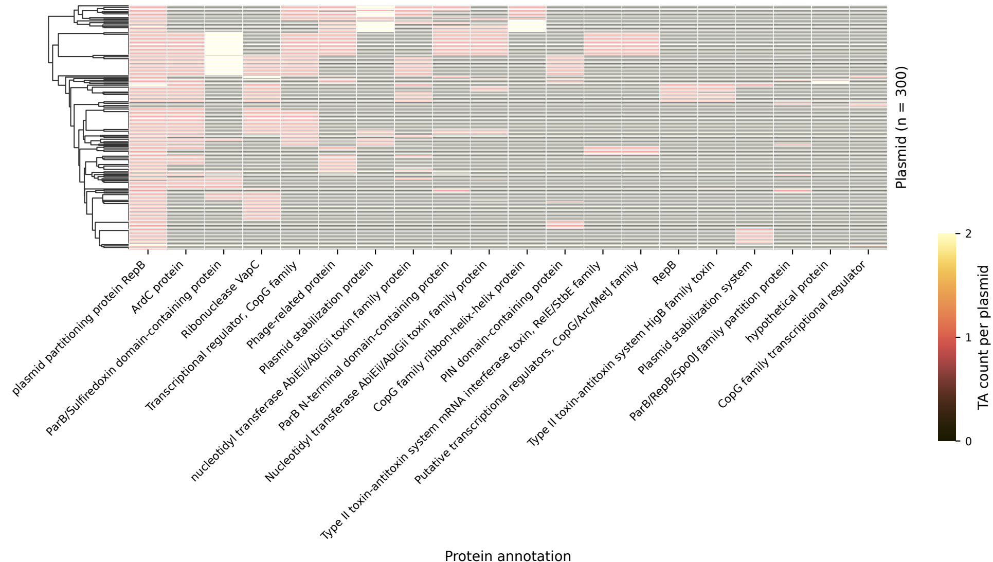
TA-system annotation composition per plasmid (top 20)
