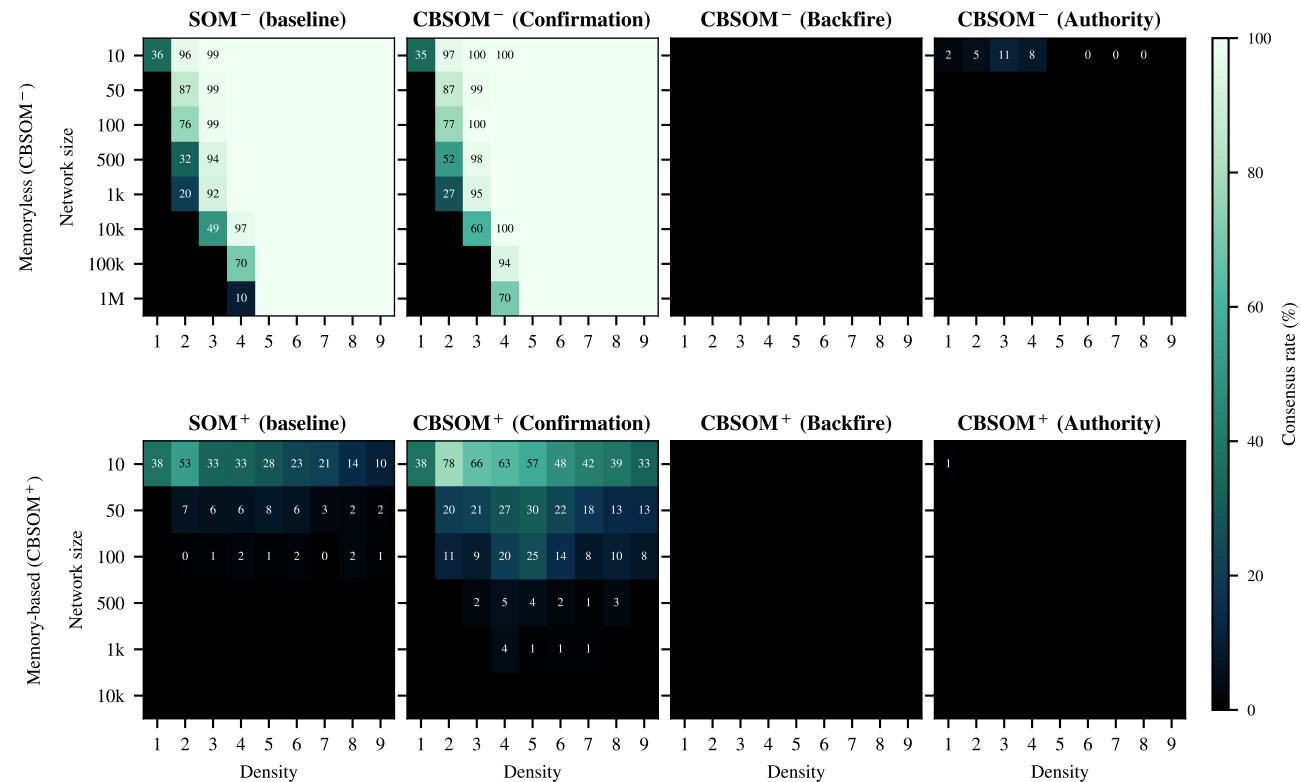
Consensus rate — uniform networks (density 1–9 × network size)
