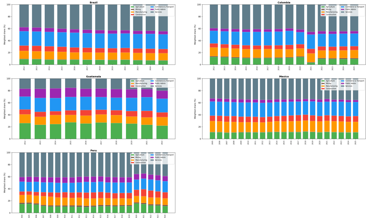
Figure 3: Industry Composition
