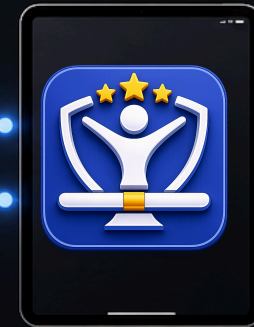
Judge C
