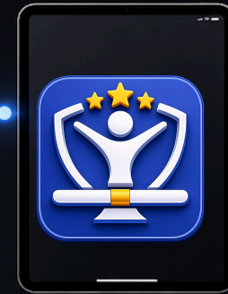
Judge A
