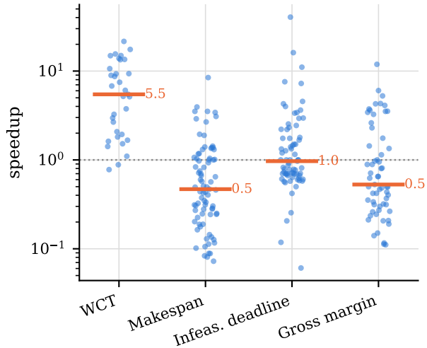
Time (no-SBS / DFA)
