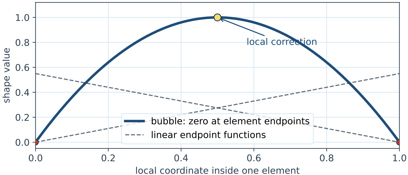
Bubble enrichment on one element
