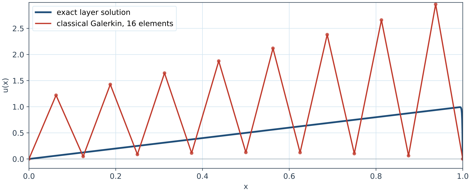
Advection dominated case: \varepsilon = 10^{-3} , \beta = 1 , f = 1
