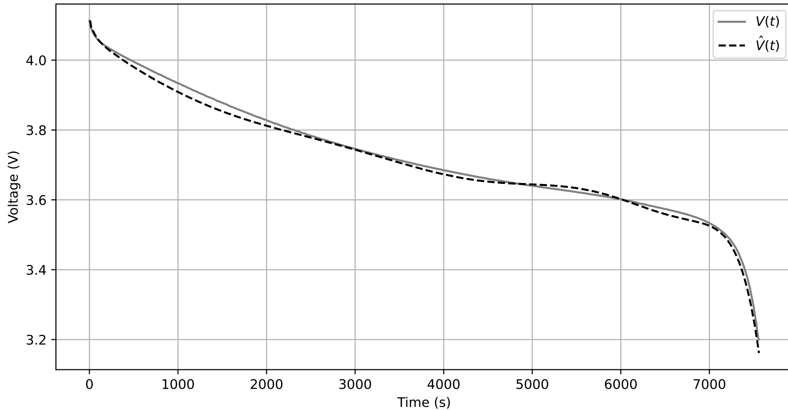
Battery Voltage Estimation using UKF @ 1.0 (A)
