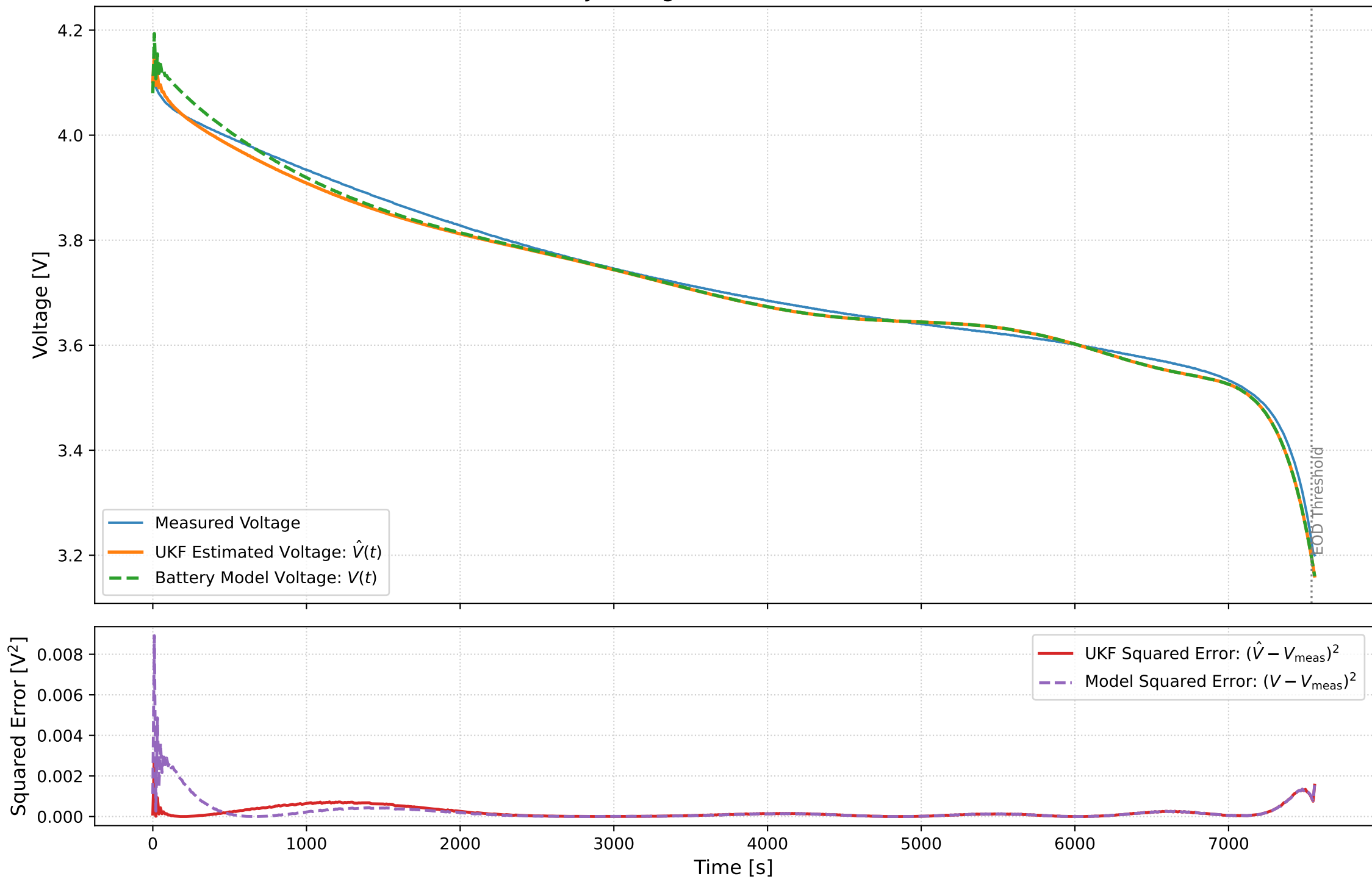
UKF Battery Voltage Estimation vs Ground Truth
