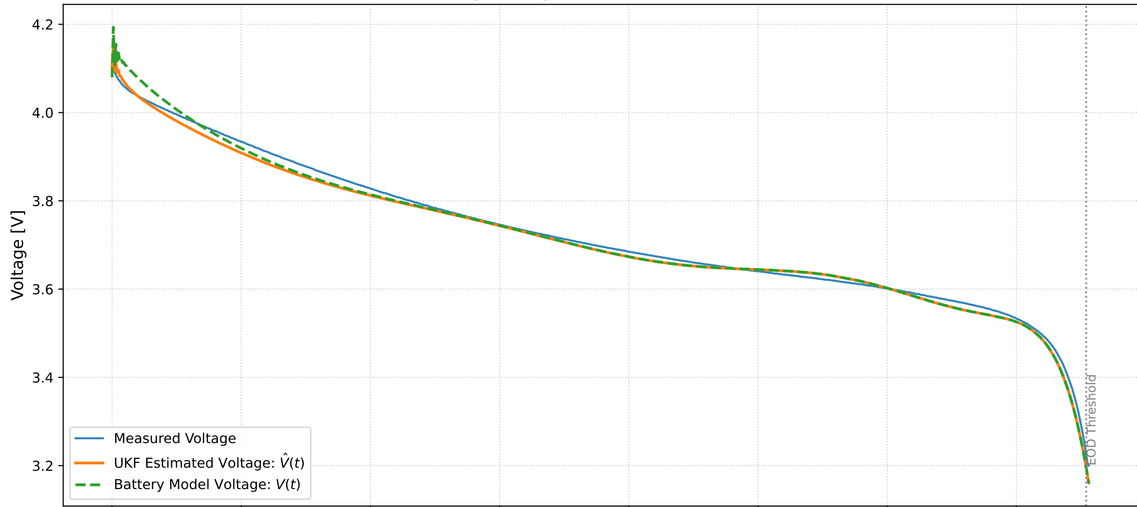
UKF Battery Voltage Estimation vs Ground Truth
