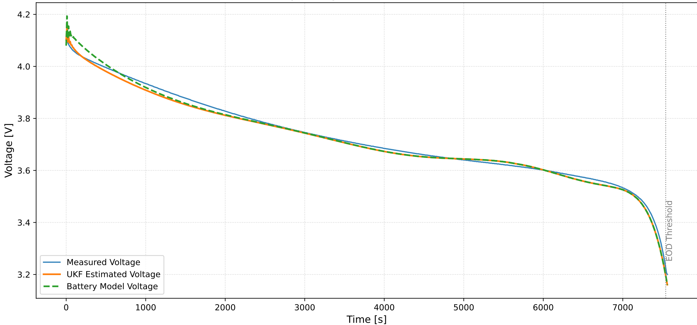
UKF Battery Voltage Estimation vs Ground Truth
