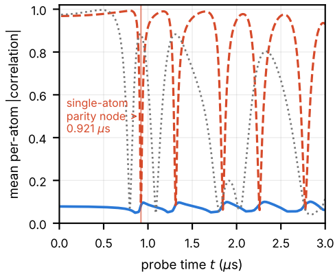
(a) V = 0 (non-interacting)
