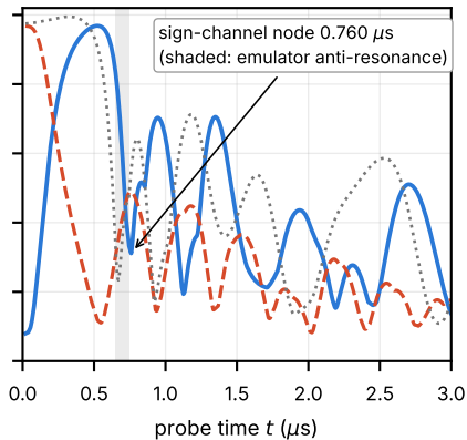
(b) V = 5.42 \text{ rad}/\mu\text{s} ( a = 10 \mu\text{m} )
