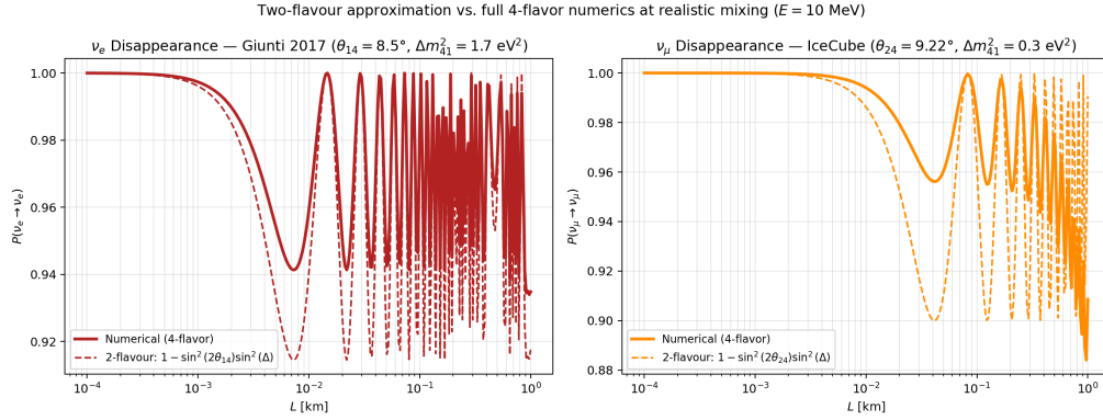
Figure 4.2: sterile2_kinematics.ipynb , k_fig4_realistic_mixing.png : numerical vs. 2-flavour survival probability at realistic mixing (Giunti-2017 for \nu_e , IceCube for \nu_\mu ), the source of the confirmed realistic-mixing table above.
