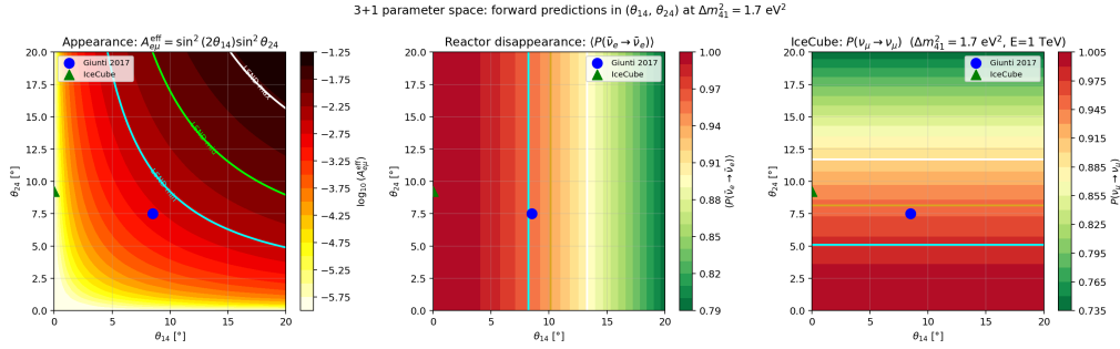
Figure 4.3: sterile3_analysis.ipynb , st2_fig7_tension.png : (\theta_{14}, \theta_{24}) contour maps (appearance amplitude, reactor rate ratio, IceCube rate) with the Giunti-2017 and IceCube benchmark points marked, illustrating the confirmed global 3+1 tension argument above.
