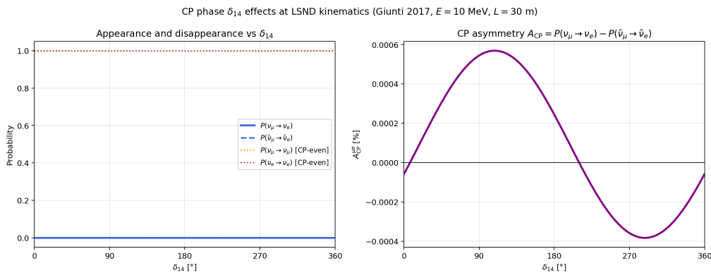
Figure 4.1: sterile1_test.ipynb , st1_fig9_cp_phase.png : \nu_\mu \rightarrow \nu_e/\bar{\nu}_\mu \rightarrow \bar{\nu}_e/\nu_\mu \rightarrow \nu_\mu/\nu_e \rightarrow \nu_e probabilities and the CP asymmetry A_{CP} against \delta_{14} at LSND kinematics, the source of the confirmed CP-scan result above.
