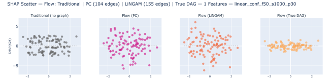
Figure 6: Shapley Flow SHAP scatter for X24 (Synthetic). Traditional shows a stable attribution pattern; both discovered-graph columns diverge substantially from the True-DAG oracle—the instance-level signature of out-degree inflation ( \Delta M_{\text{base}} = 32.5\% of \hat{\sigma} ).
