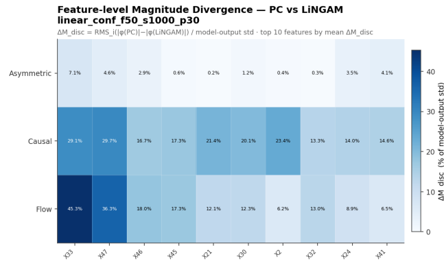
(a) Synthetic. Asymmetric near-zero; Causal and Flow concentrate on X33 and X47.
