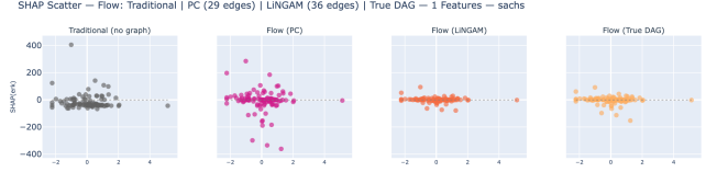
Figure 7: Shapley Flow SHAP scatter for erk (Sachs). All three graph-aware variants diverge from each other and from Traditional. Flow+PC inflates erk’s attributions by treating it as an isolated source node; only Flow+True DAG tracks the correct downstream credit distribution.
