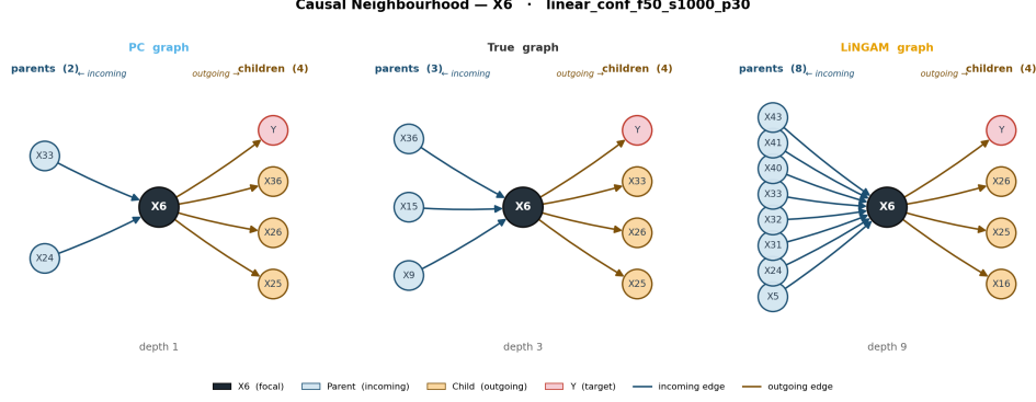
Figure 23: Causal neighbourhood of X6 across the PC (left), True DAG (centre), and LiNGAM (right) graphs, synthetic dataset. X6 is a genuine intermediate node with 3 incoming and 4 outgoing edges in the True DAG. LiNGAM inflates its in-degree to 8, the over-connection that contaminates its interventional parent set under Causal Shapley.
