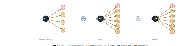
Figure 9: Causal neighbourhood of X21 (Synthetic). In the True DAG and under PC the edge runs X_{21} \rightarrow X_{47} . LiNGAM reverses it to X_{47} \rightarrow X_{21} , misdirecting attribution credit in both CSV and Flow.
