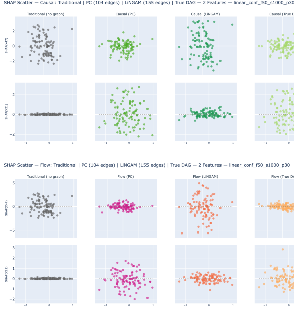
Figure 10: SHAP scatter for X21 and X47 (Synthetic). Top (Causal Shapley): under PC both features track the oracle; under LiNGAM, X47 is suppressed and X21 acquires inflated credit. Bottom (Shapley Flow): the same orientation-driven credit transfer appears; Flow+PC and Flow+True agree closely while Flow+LiNGAM diverges on both features.
