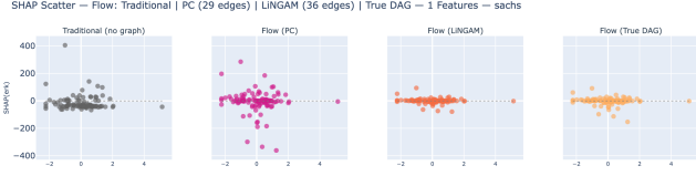
Figure 12: SHAP Flow SHAP scatter for erk (Sachs). All three graph-aware variants diverge from each other and from Traditional. Flow+PC inflates erk’s attributions by treating it as an isolated source node; only Flow+True DAG tracks the correct downstream credit distribution.
