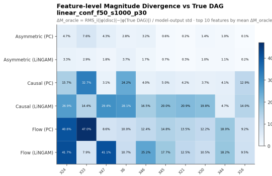
(a) Synthetic dataset (top 10 features by mean \Delta M_{\text{oracle}} ). Asymmetric rows are near-zero; Causal and Flow concentrate their oracle deviations on X24, X33, and X47.
