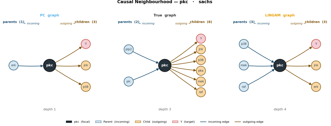
Figure 26: Causal neighbourhood of pkc across the PC (left), True DAG (centre), and LiNGAM (right) graphs, Sachs dataset. PC and LiNGAM discover different parent and child sets for pkc , generating different interventional conditioning environments. Because pkc ’s Traditional Shapley values sit near zero, these structural differences are sufficient to produce high sign disagreement without producing large magnitude divergence.
