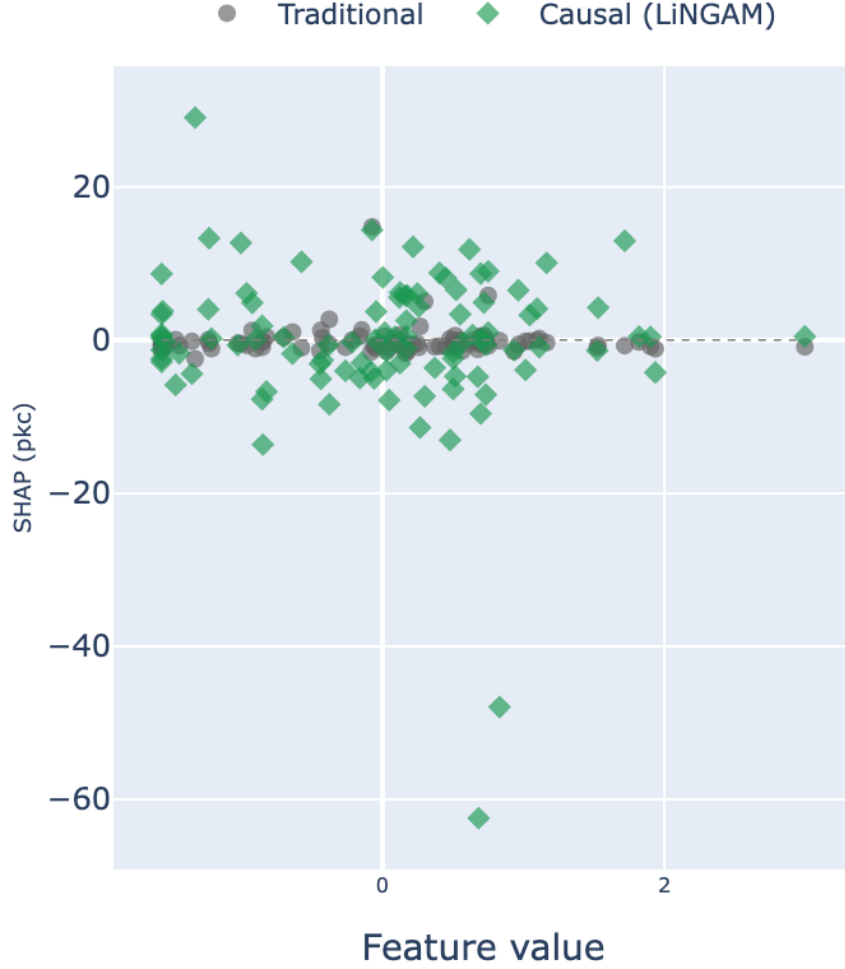
Figure 27: Traditional vs. Causal+LiNGAM SHAP scatter for pkc, Sachs dataset. The Traditional column concentrates near zero; Causal+LiNGAM disperses attributions to both sides of zero. The magnitude of the shift is small relative to \hat{\sigma} , which is why pkc does not appear in the magnitude heatmaps, but it is large enough to cross the sign boundary for a high fraction of instances, which is precisely why it leads the sign heatmaps instead.
