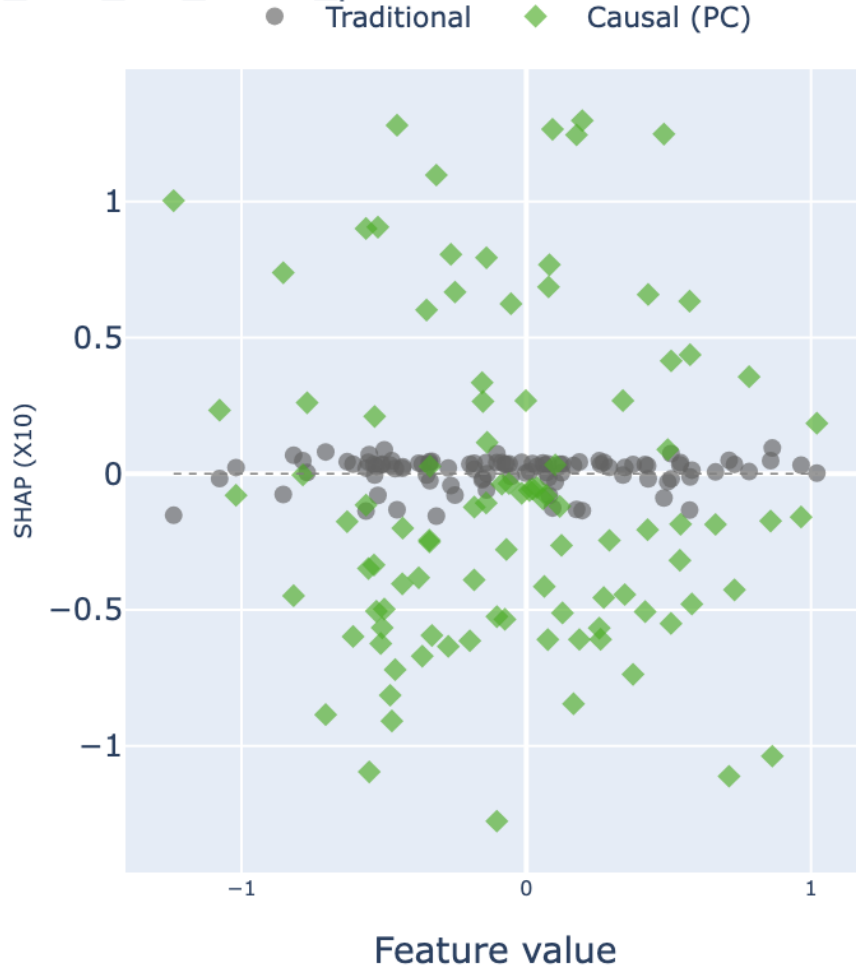
Figure 25: Traditional vs. Causal+PC SHAP scatter for X10, synthetic dataset. The Traditional column shows attributions clustered near zero; the Causal+PC column disperses them to both sides of zero with larger magnitude. This scatter-level divergence, producing D_{\text{base}} = 96\% , is the direct consequence of near-zero baseline attributions being pushed across the sign boundary by graph-induced interventional redistribution.
