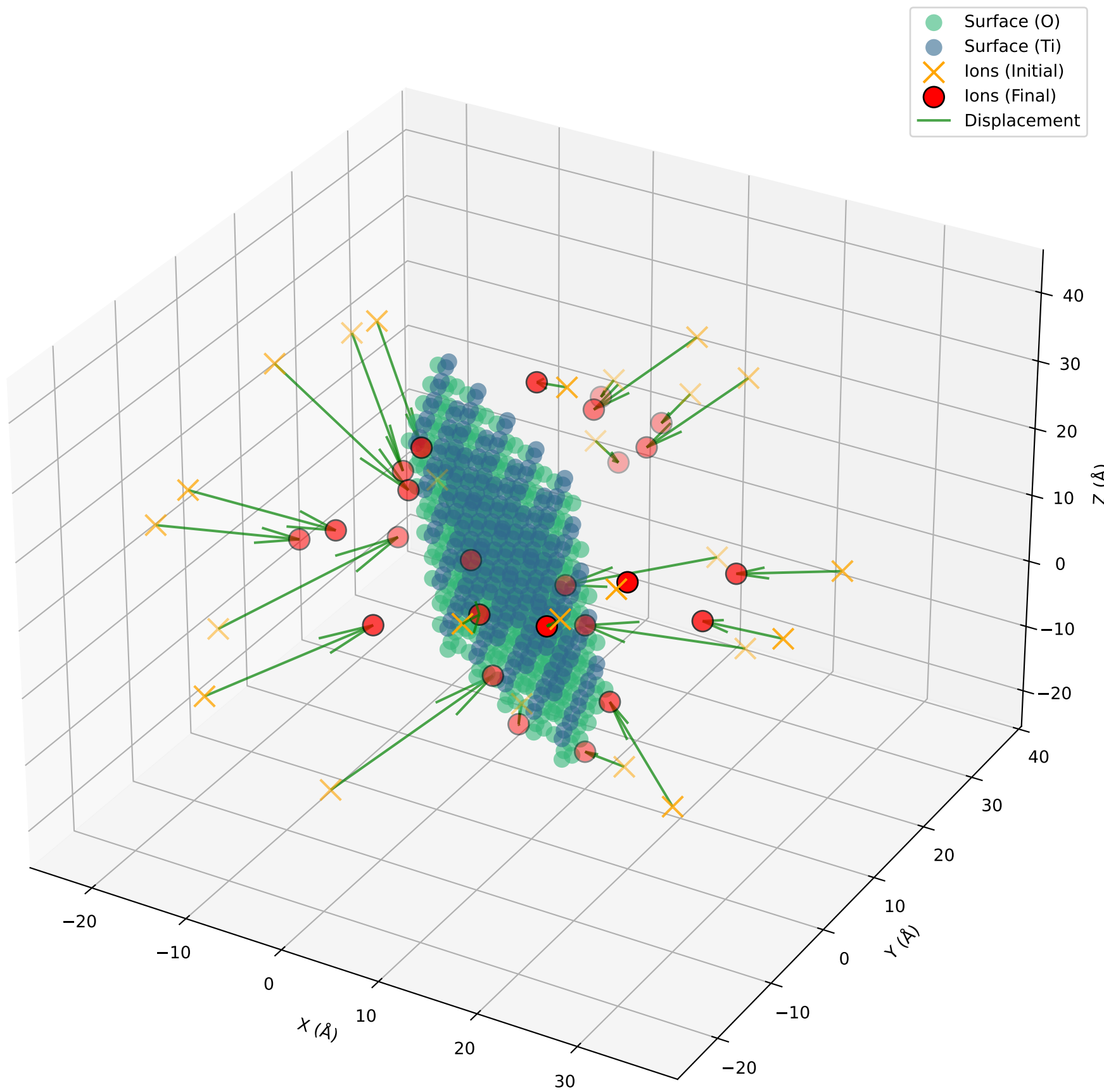
Initial and Final Ion Positions for TiO 2 _bulk_anatase_control_small
