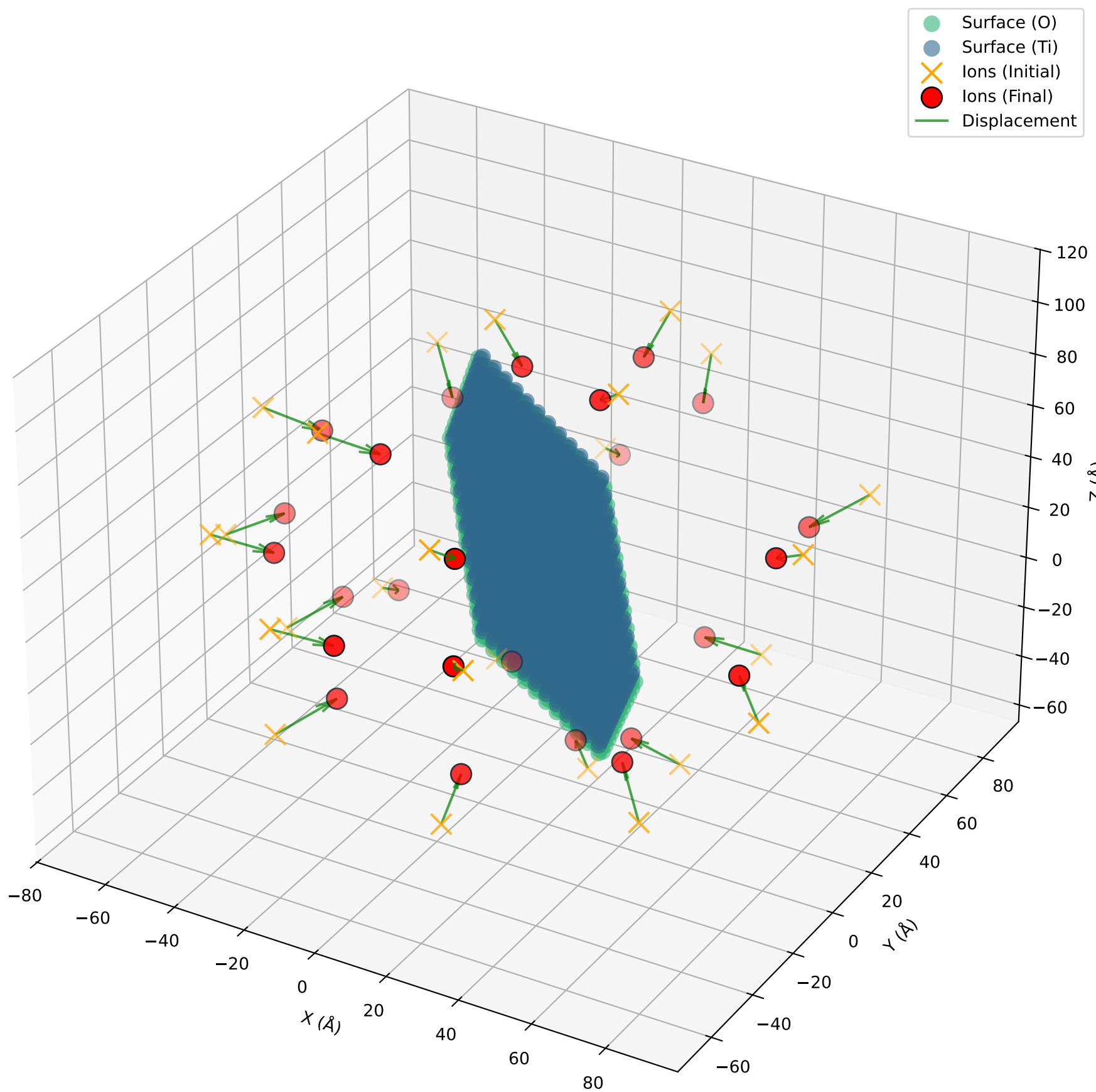
Initial and Final Ion Positions for TiO2_bulk_anatase_No_Kmeans
