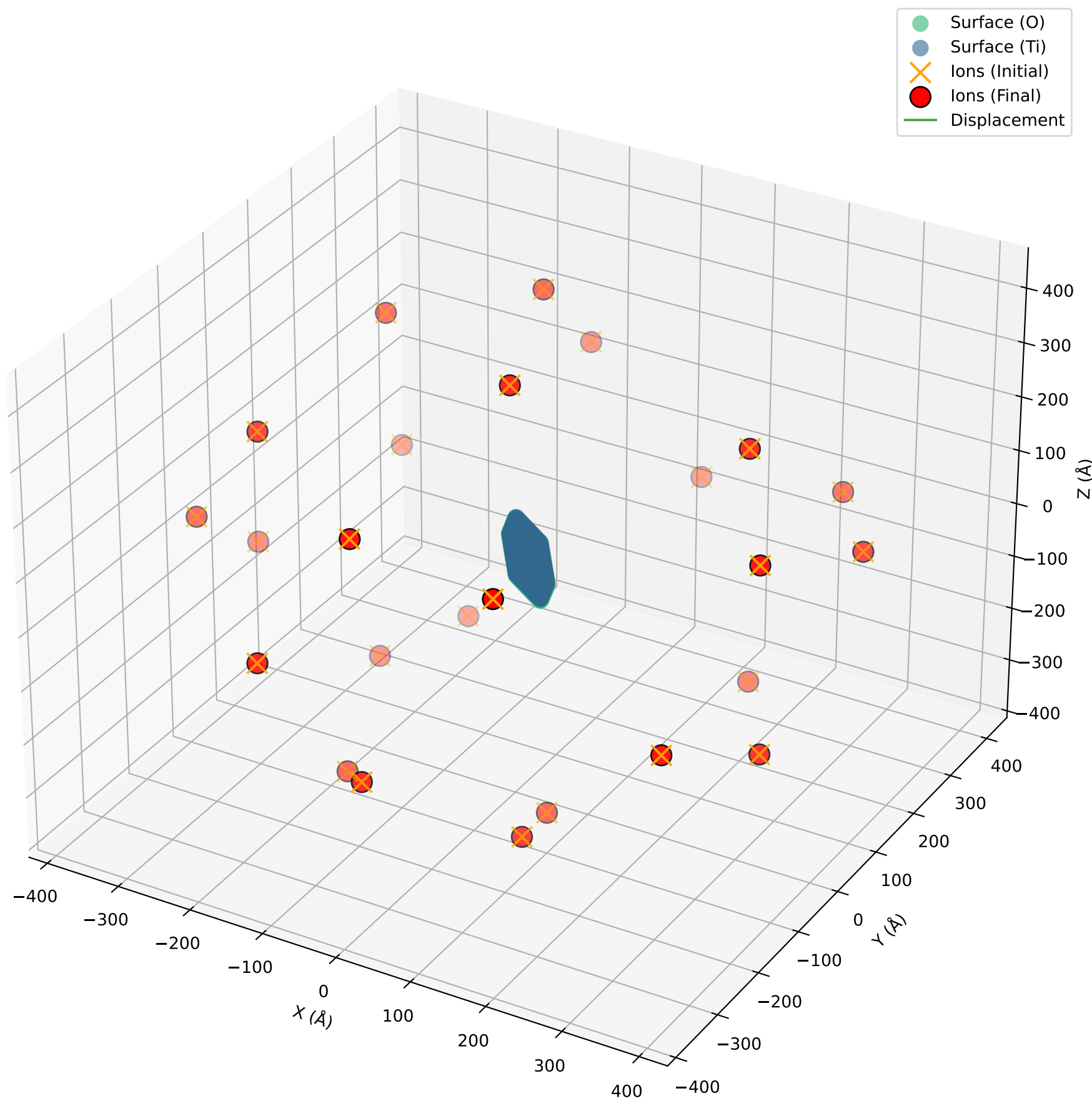
Initial and Final Ion Positions for TiO 2 _bulk_anatase_No_Optuna
