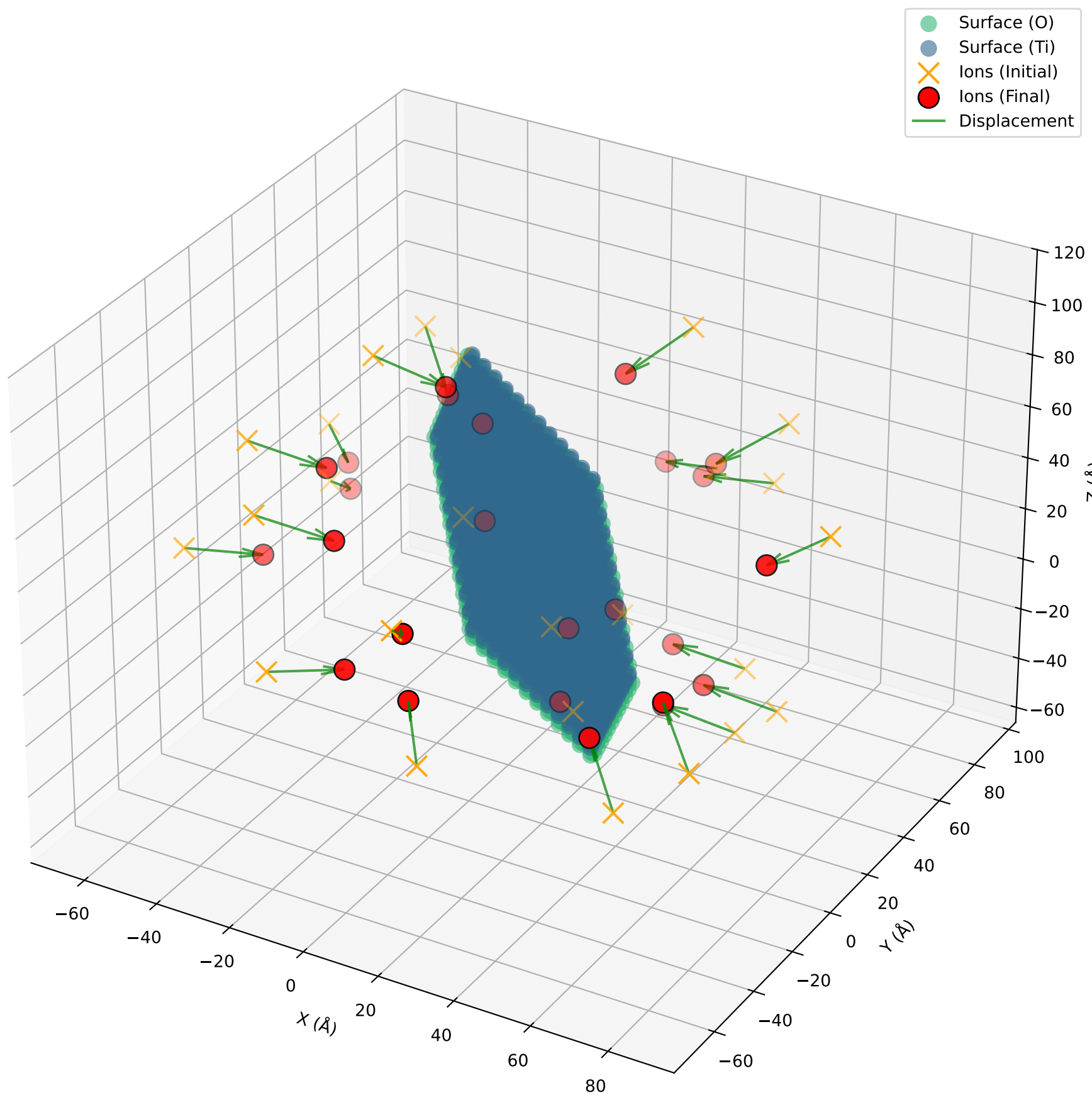
Initial and Final Ion Positions for TiO 2 _bulk_anatase_control_big
