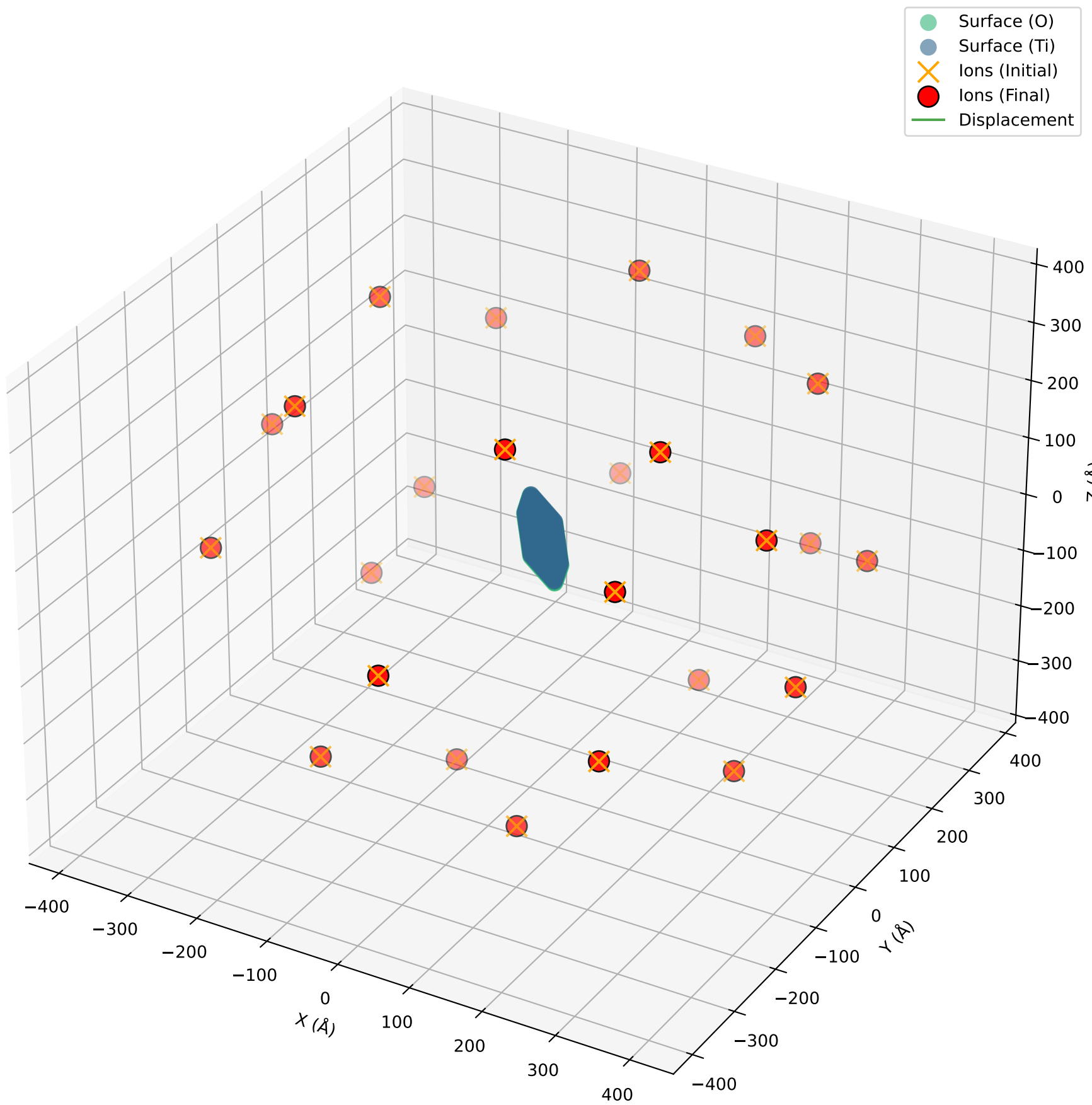
Initial and Final Ion Positions for TiO2_bulk_anatase_only_optuna
