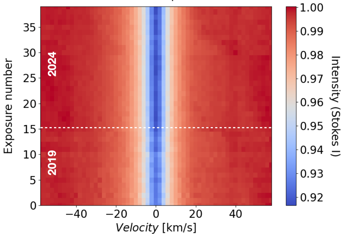
LSD Stokes I profiles
