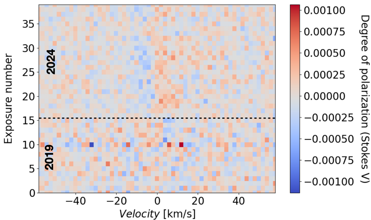
LSD Stokes V profiles
