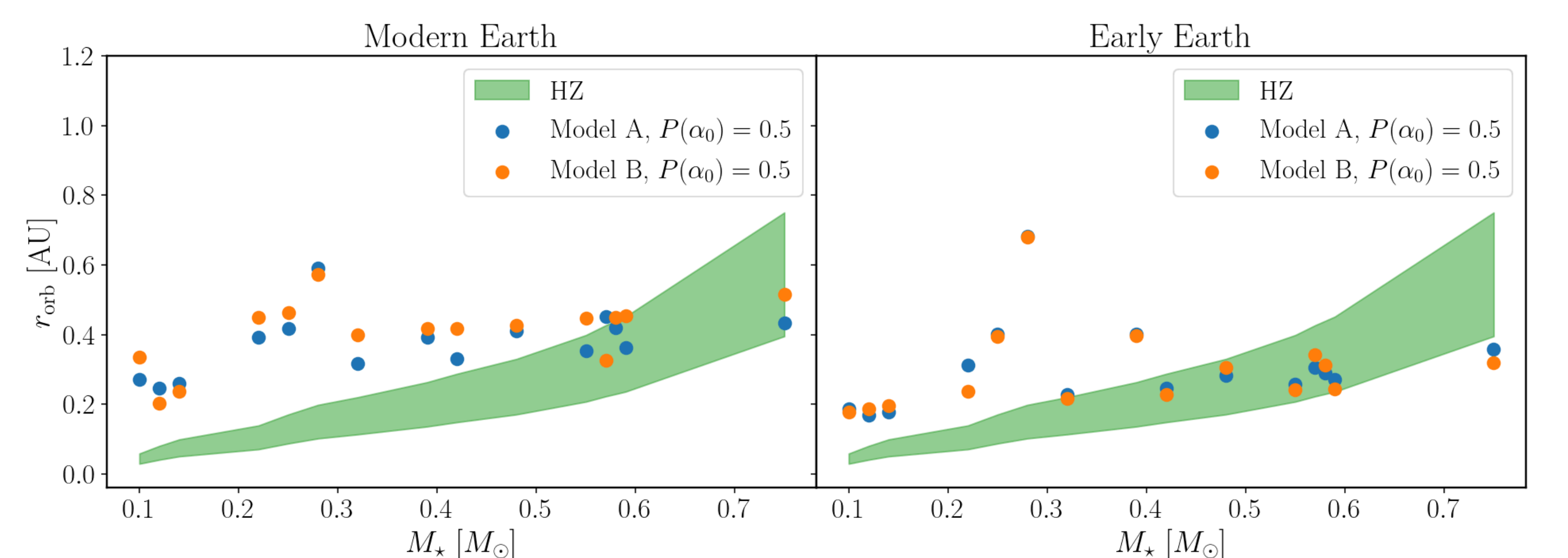
Figure 4. Orbital distance required for a specific atmospheric protection likelihood of 0.5, as a function of mass.
